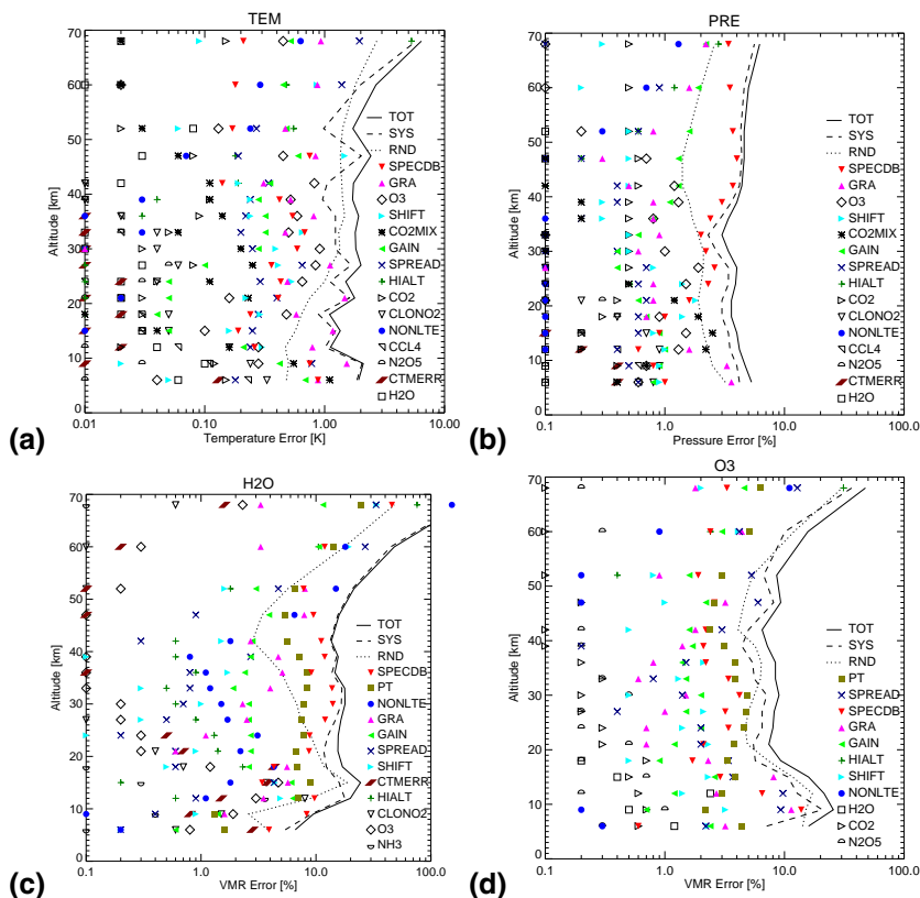
Fig. 7. Error budgets for the MIPAS retrievals of temperature, pressure, water vapour and ozone computed are for midlatitude daytime conditions. The solid line is the Total Error (or Accuracy), represented by the rootsumsquare of the Random Error (or Precision), shown as the dotted line, and the forward model errors, shown as the dashed line. The forward model error is itself the rootsumsquare of the various components shown by different symbols (see Table 3 for details).
