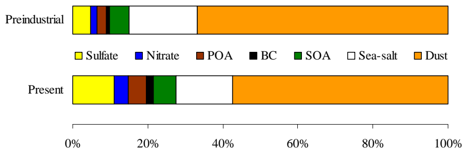
Fig. 3. Contribution to the total aerosol optical depth for each one of the aerosol species (annual global mean) for the preindustrial (top; AOD 0.084) and present (bottom; AOD 0.102) atmospheres. Ammonium aerosol is included in the nss-sulfate and nitrate contribution.
