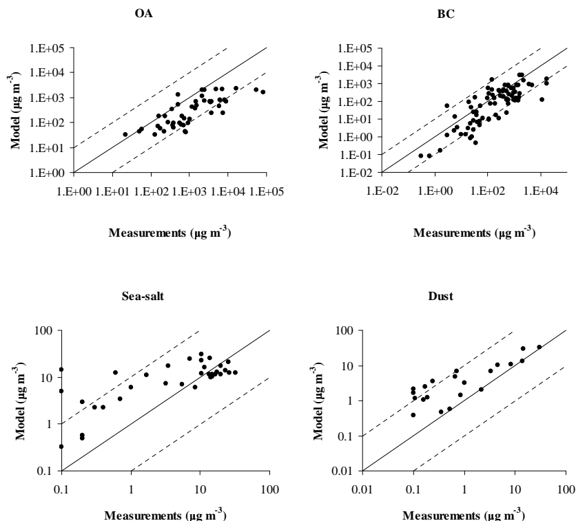
Fig. 1. Measured vs. modeled OA (top-left), BC (top-right), sea-salt (bottom-left) and dust (bottom-right) values for the present day. The solid line denotes the 1:1 ratio and the dashed lines the 1:10 and 10:1 ratios, respectively. Dust and sea-salt measurements are annual means from the European measurement network EMEP ( http://www.emep.int ), the North-American measurement network IMPROVE ( http://vista.cira.colostate.edu/improve ) and measurements compiled by the Global Atmosphere Watch (GAW) program ( http://wdca.jrc.it ). Carbonaceous aerosol measurements are those used in Tsigaridis and Kanakidou (2003).
