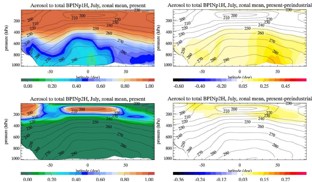
Fig. 9. Ratio of aerosol-phase to aerosol- and gas-phase SOA species (zonal mean) for the present (left panels) and the corresponding difference from the preindustrial (right panels) simulation for BPINp1H (top panels) and BPINp2H (bottom panels). Contours show the zonal mean temperature (K). Note the different scale between the two panels on the right.
