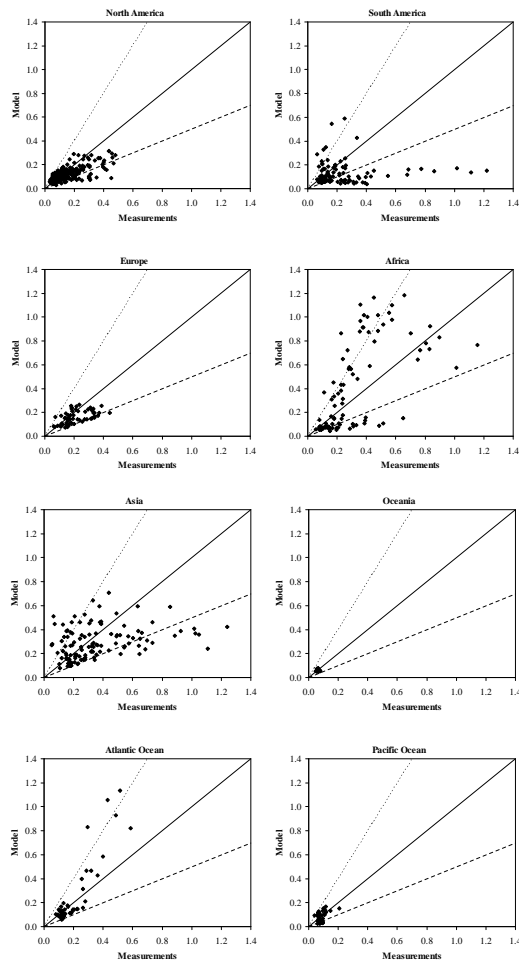
Fig. 2. AOD results vs. measurements (500 nm) from the AERONET network ( http://aeronet.gsfc.nasa.gov ) separated by region. The solid line denotes the 1:1 ratio and the dotted lines the 1:2 and 2:1 ratios, respectively.
