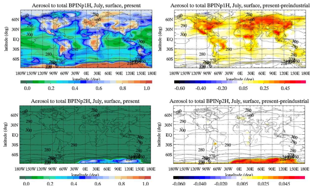
Fig. 8. Ratio of aerosol-phase to aerosol- and gas-phase SOA species (surface) for the present (left panels) and the corresponding difference from the preindustrial (right panels) simulation for BPINp1H (top panels) and BPINp2H (bottom panels). Contours show the monthly mean temperature (K).
