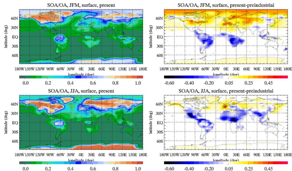
Fig. 7. SOA to OA mass surface ratio for winter (top panels) and summer (bottom panels) for the present (left panels) and the corresponding difference from the preindustrial (right panels) simulation.
