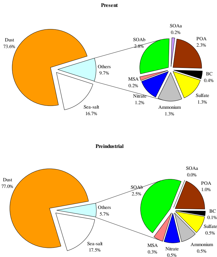
Fig. 5. Relative contribution of aerosol components to the total aerosol burden for the present (top) and preindustrial atmospheres (bottom) based on the model calculations. The total aerosol burden is 28.9 Tg and 26.8 Tg, respectively.
