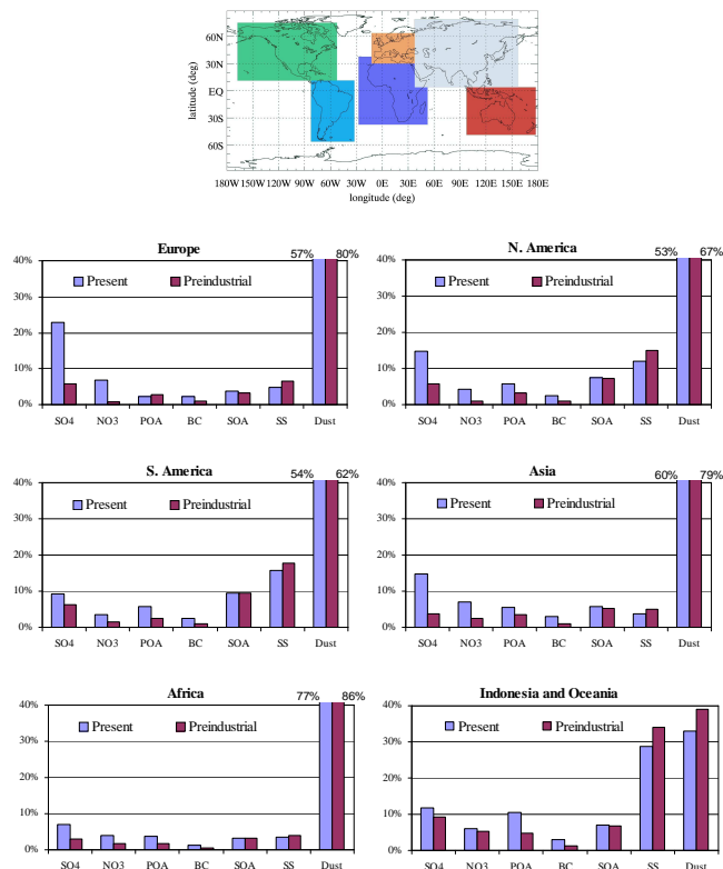
Fig. 4. Map: Continental box regions definition for the AOD comparison. The African box overlaps with the European and the Asian ones. Charts: Relative percentage contribution of aerosol components per continent for the present and preindustrial atmospheres. The effect of water is included to each one of the aerosol components. The continental mean AOD values for the present and preindustrial simulations, respectively, are: Europe: 0.204, 0.146; N. America: 0.092, 0.074; S. America: 0.099, 0.087; Asia: 0.179, 0.136; Africa: 0.311, 0.279; Indonesia and Oceania: 0.071, 0.060. SS means sea-salt.
