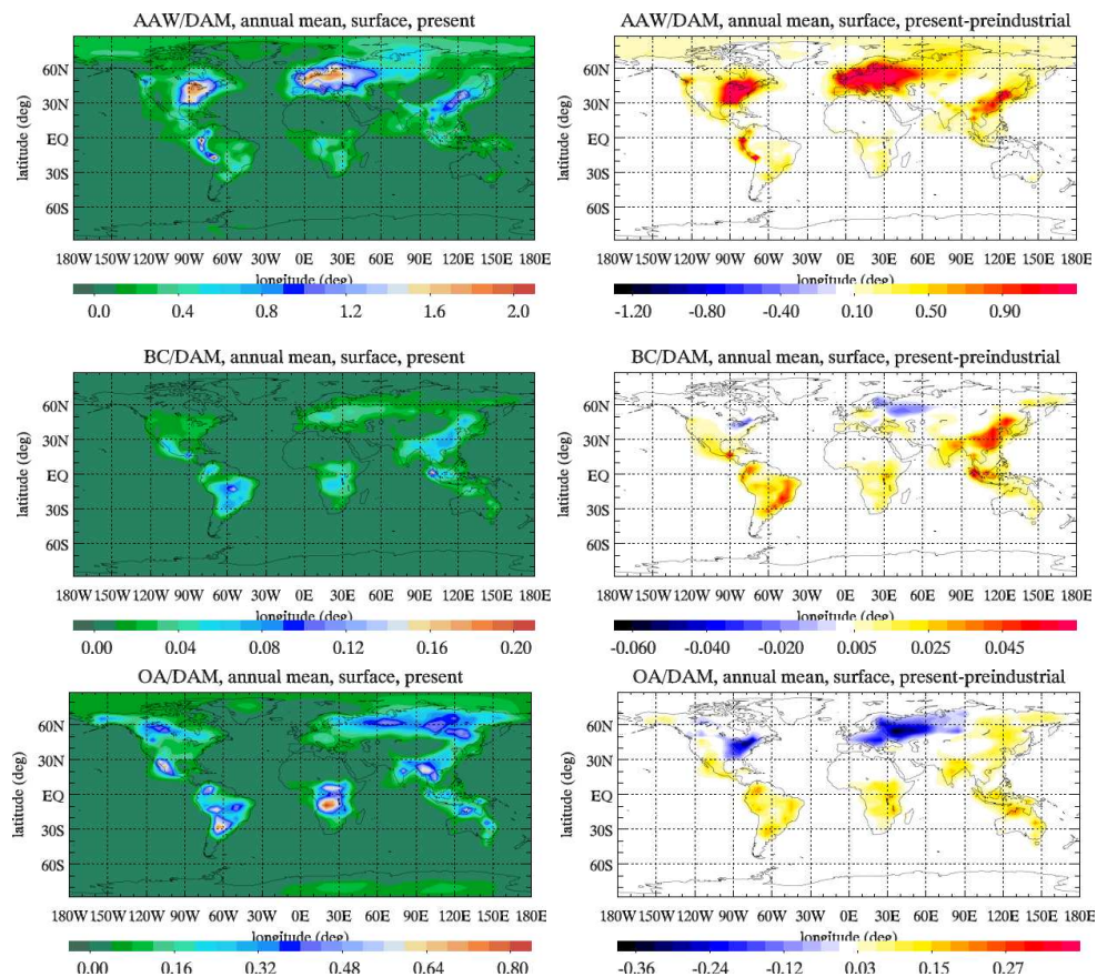
Fig. 6. Annual mean aerosol component to dry aerosol mass (DAM) surface ratio for the present (left panels) and the corresponding difference from the preindustrial (right panels) simulation. Aerosol components are AAW (top panels) BC (medium panels) and OA (bottom panels).
