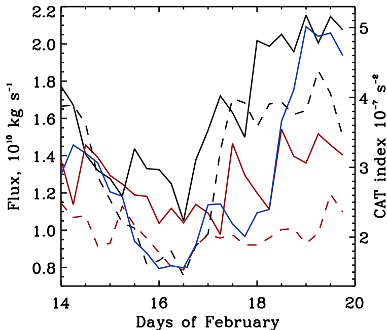
Fig. 7. Time series of CAT index and absolute values of downward and upward CTF averaged over the domain 310° W–60° E and 60° N–85° N. Solid lines are CTF calculated from analyses; dashed lines are those from forecasts. Downward CTF is black, upward CTF is red, CAT index is blue.
