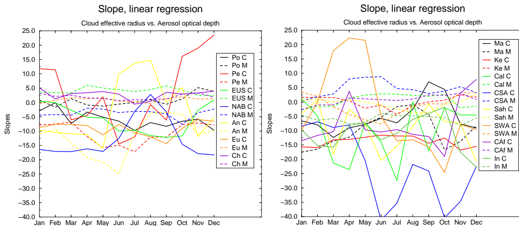
Fig. 8. Slopes for the linear regression of Aerosol Optical Depth vs. Cloud Effective Radius for the 15 regions for both MODIS and CAM-Oslo.
