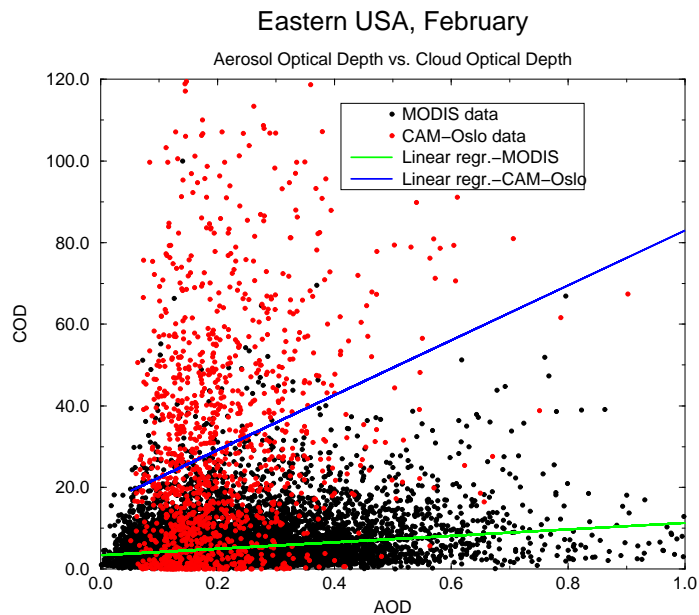
Fig. 4. Liquid Cloud Optical Depth as a function of Aerosol Optical Depth for Eastern USA in February for both MODIS and CAM-Oslo data.
