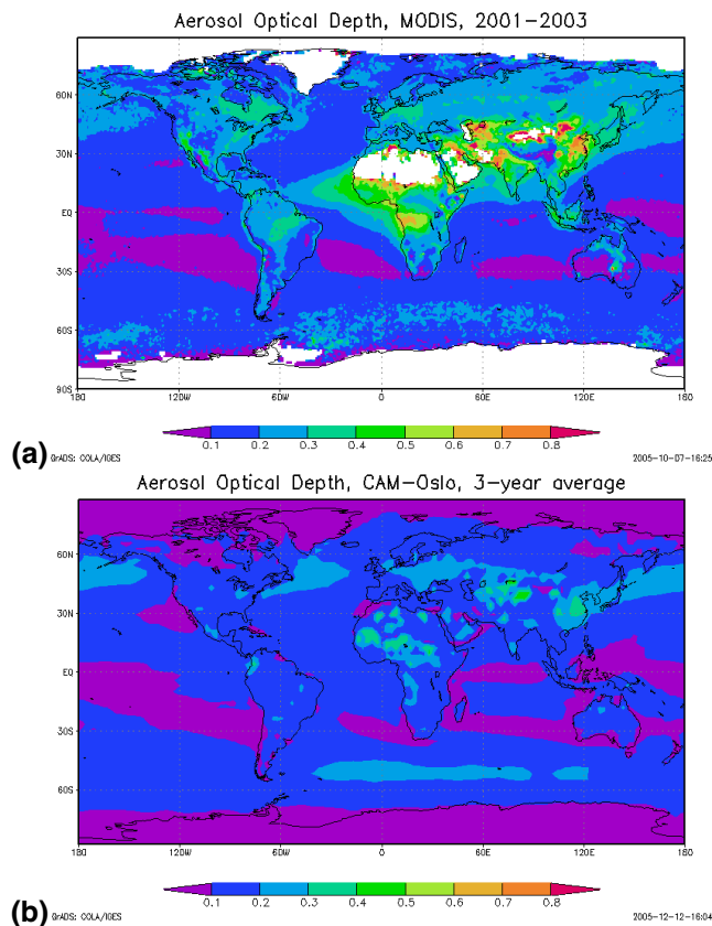
Fig. 10. Global maps of Aerosol Optical Depth from (a) MODIS and (b) CAM-Oslo.
