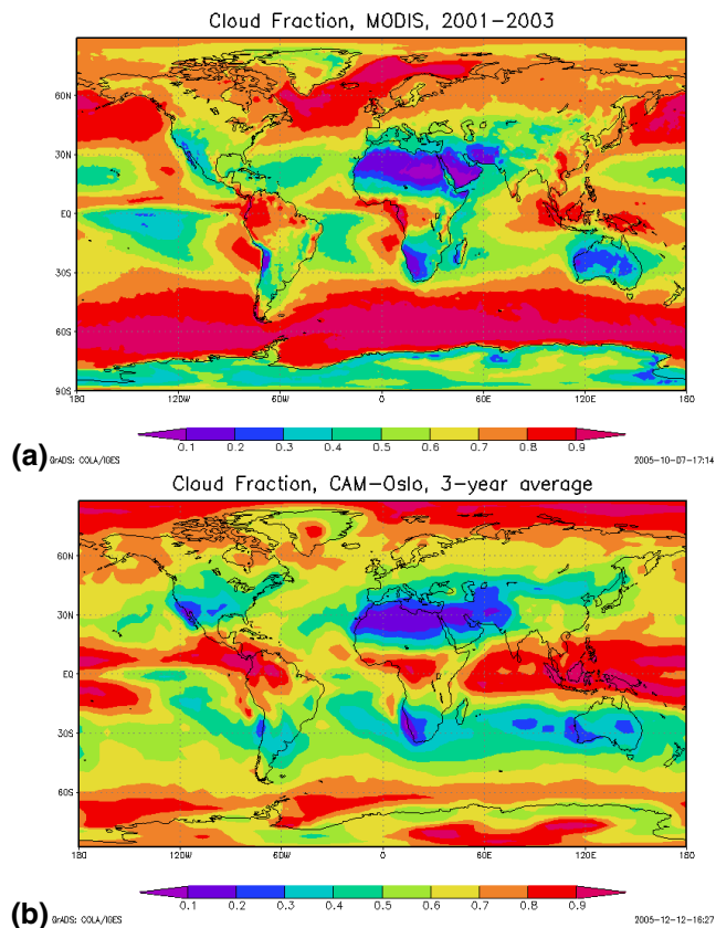
Fig. 11. Global maps of total cloud fraction from (a) MODIS and (b) CAM-Oslo.
