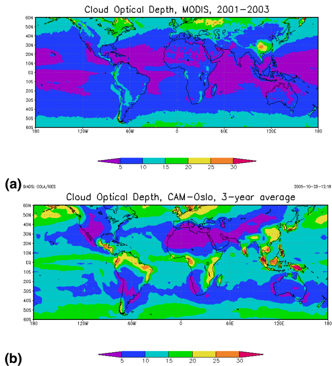
Fig. 14. Global maps of Liquid Cloud Optical Depth from (a) MODIS and (b) CAM-Oslo.
