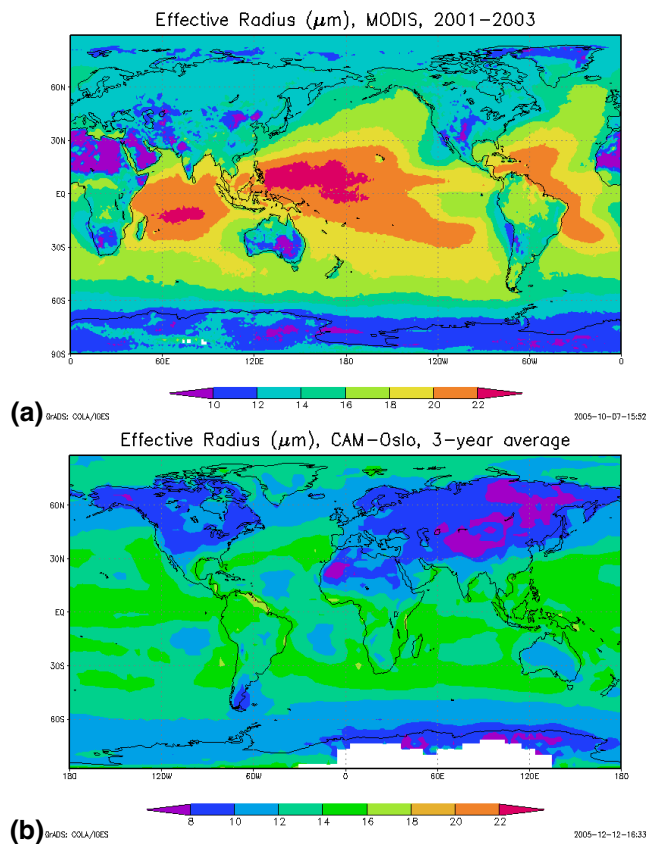
Fig. 12. Global maps of Cloud Droplet Effective Radius from (a) MODIS and (b) CAM-Oslo.
