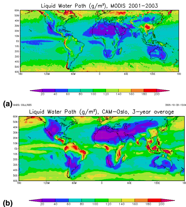
Fig. 13. Global maps of Liquid Water Path from (a) MODIS and (b) CAM-Oslo.
