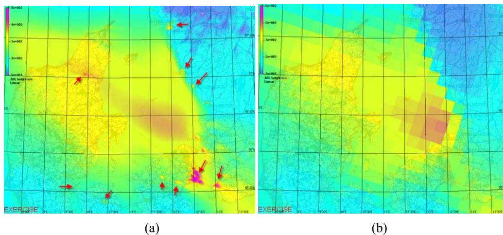
Fig. 8. The mixing height for a large part of Denmark as calculated from different versions of DMI-HIRLAM: (a) urbanised U01, (b) operational T15. Main cities are shown by arrows.
