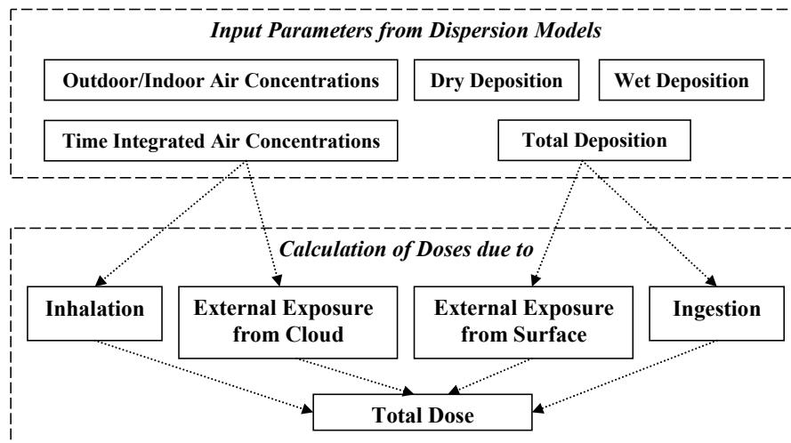
Fig. 6. General scheme of individual dose calculations for different groups of the population from radioactive airborne contamination in the ARGOS system.
