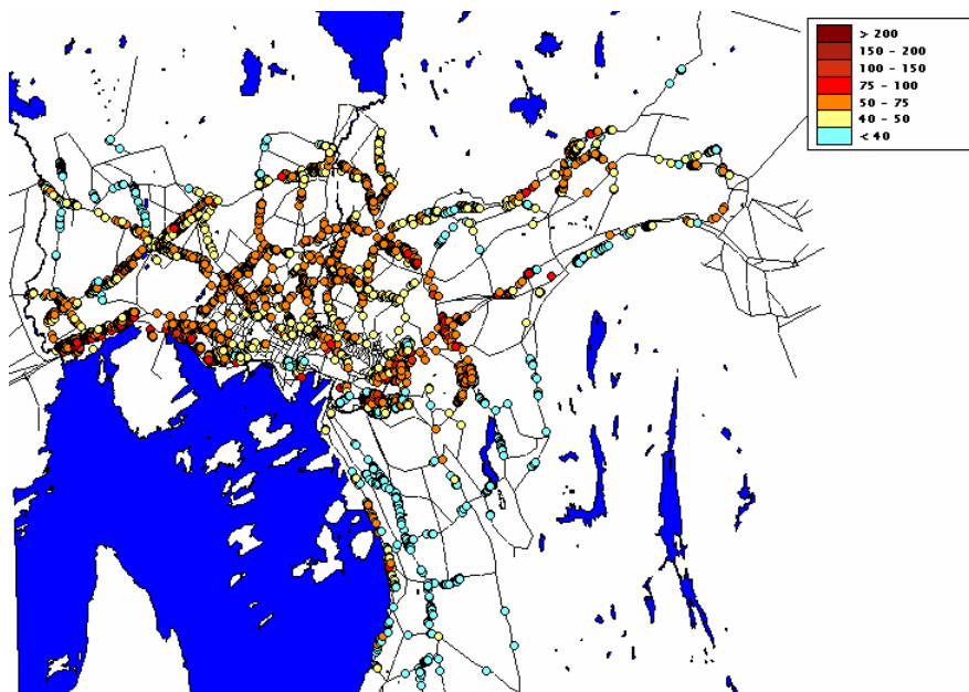
Fig. 4. Example of hourly concentration distribution of PM 10 in the selected “building points” ( \mu\text{g}/\text{m}^3 ).
