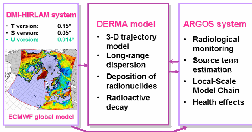
Fig. 5. Structure of the Danish nuclear emergency modelling system.
