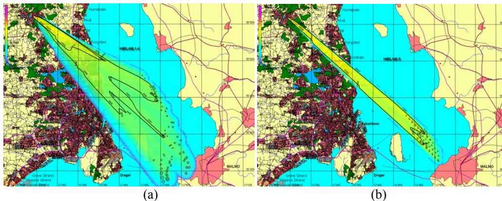
Fig. 7. A local-scale plume from the ^{137}\text{Cs} hypothetical atmospheric release in Hillerød at 00:00 UTC, 19 June 2005 as calculated with RIMPUFF using DMI-HIRLAM and visualised in ARGOS for the Copenhagen Metropolitan Area. Cs-137 air concentration for different DMI-HIRLAM data: (a) urbanised U01, 1.4 km resolution, (b) operational S05, 5 km resolution.
