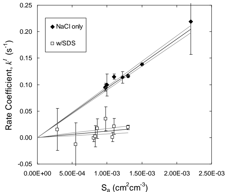
Fig. 3. Corrected first order rate constants for reaction of \text{N}_2\text{O}_5 with NaCl aerosol ( \blacklozenge ) and reaction with NaCl aerosol containing 10 wt% SDS ( \square ) as a function of measured aerosol surface area. Lines shown represent weighted linear least squares fits to the data, with confidence limits of 1\sigma . For all experiments shown, \sim 22 ppb \text{N}_2\text{O}_5 was present initially. Data obtained at 51%, 62%, and 72% RH are shown.
