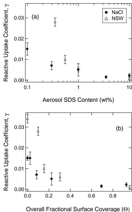
Fig. 4. Reaction probability, \gamma^{\text{N}_2\text{O}_5} , is plotted (a) versus SDS concentration in the aerosol and (b) as a function of overall fractional SDS surface coverage in the aerosol population, assuming 1 monolayer = 2 \times 10^{14} molecules \text{cm}^{-2} (see text for details). Data shown is for reaction of \sim 22 ppb \text{N}_2\text{O}_5 with NaCl and natural seawater (NSW) aerosols at 60% RH.
