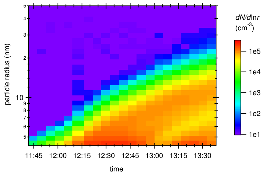
Fig. 2. Evolution of measured size distributions. Colour indicates particle number density. Lights were turned on at 11:09; additional \text{SO}_2 injections took place at 11:59 and 12:50.
