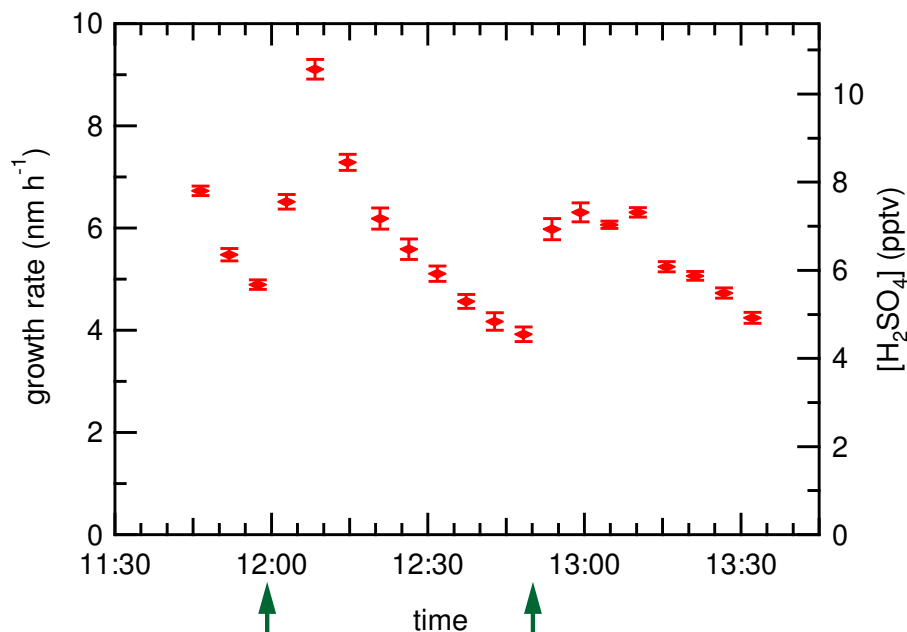
Fig. 3. The particle growth rate determined using PARGAN. The growth rate is proportional to the \text{H}_2\text{SO}_4 concentration (see Eq. 5), the corresponding values of which can be read off the right axis. Lights were turned on at 11:09; additional \text{SO}_2 injections took place at 11:59 and 12:50 (indicated by arrows).
