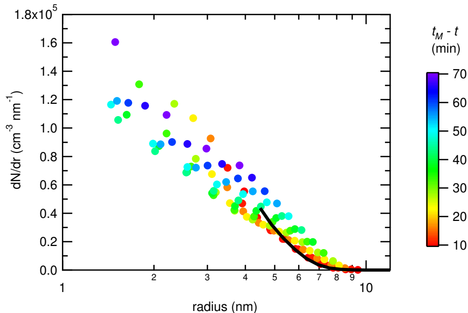
Fig. 4. Measured (solid line) and reconstructed (symbols) size distributions for 16 November 12:22. Reconstruction is based on size distributions, measured at later times. Colour of symbol indicates the magnitude of extrapolation, t_M - t .
