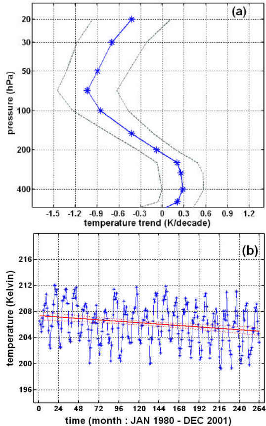
Fig. 4. (a) Linear temperature trend (in Kelvin per decade) height profile framed with the 95% confidence profiles. (b) Time evolution of the monthly averaged temperature values in the lower stratosphere (at 70 hPa), over Durban. The superimposed red line indicates the obtained linear trend, i.e., -1.09 \pm 0.27 K.
