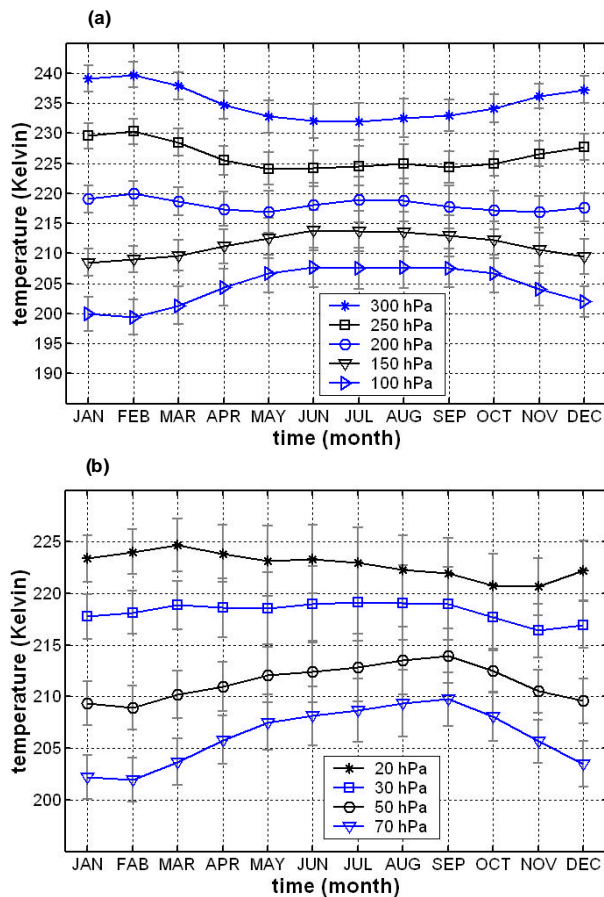
Fig. 2. Time evolution of monthly averaged temperatures per heights: (a) in the upper troposphere and (b) in the lower stratosphere over Durban (see legends).
