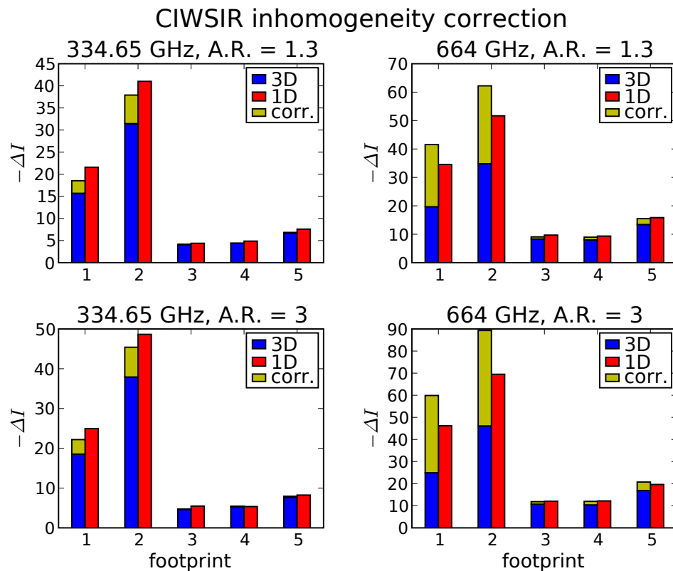
Fig. 10. Comparing the beamfilling correction in Eq. (7) against the observed differences.
