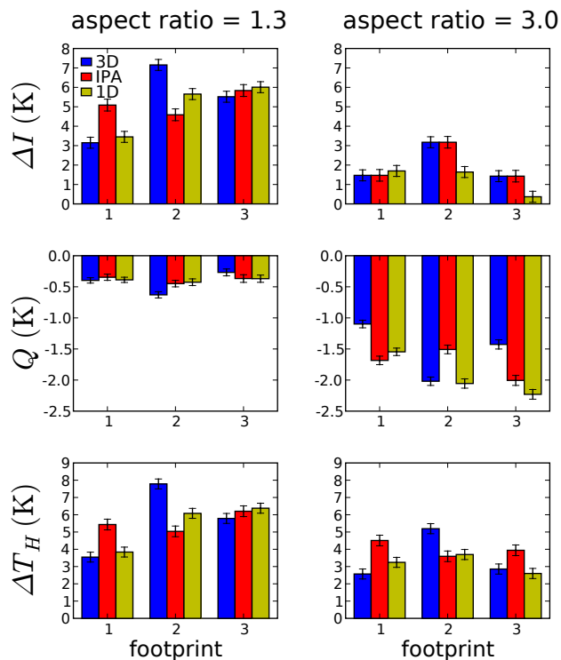
Fig. 7. Simulations results for EOSMLS, 10 km tangent height: plot layout as for Fig. 3. For 10 km tangent height the sign of the cloud induced radiance and polarisation is reversed. Agreement between 3-D, IPA and 1-D is poor.
