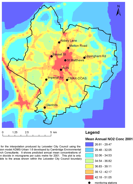
Fig. 1. Modeled NO 2 concentrations in the Leicester Area, produced by the ADMS model, using assimilated data from the automated monitoring stations marked on the map. The location of the CMAX-DOAS instrument is shown.
