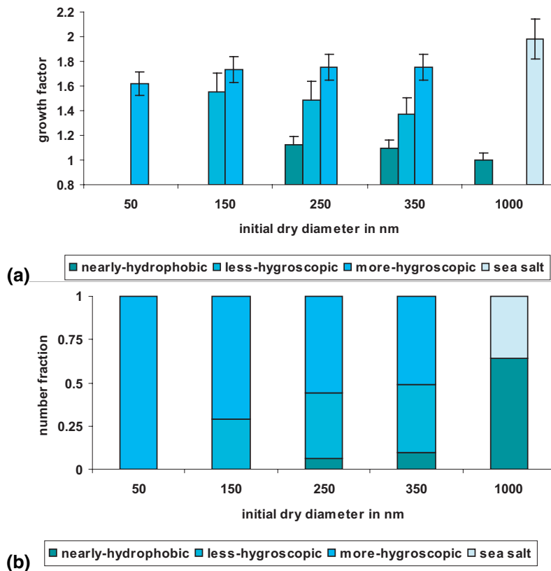
Fig. 8. (a) Hygroscopic growth factors and (b) number fractions for particles with initial dry sizes D_p=50, 150, 250, 350 nm and 1 \mu\text{m} measured at 90% RH for an air mass influenced by sources from Asian dust regions and Shanghai during period 5..
