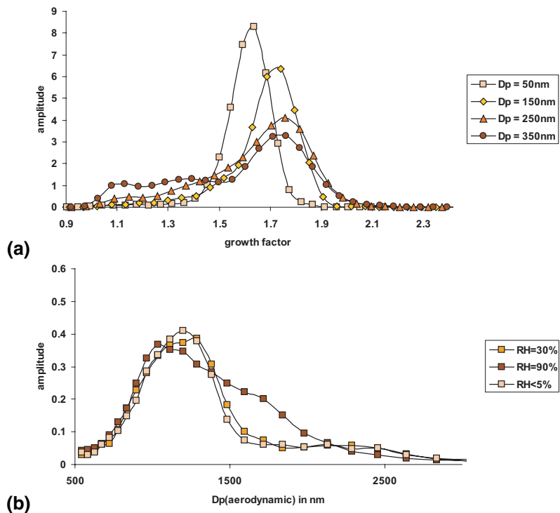
Fig. 7. Hygroscopic growth distributions for particles with an initial dry size of (a) D_p = 50, 150, 250, 350 nm measured at 90% RH and (b) D_p = 1 m measured at 90, 30, and <5% RH for an air mass influenced by sources from Asian dust regions and Shanghai during period 5.
