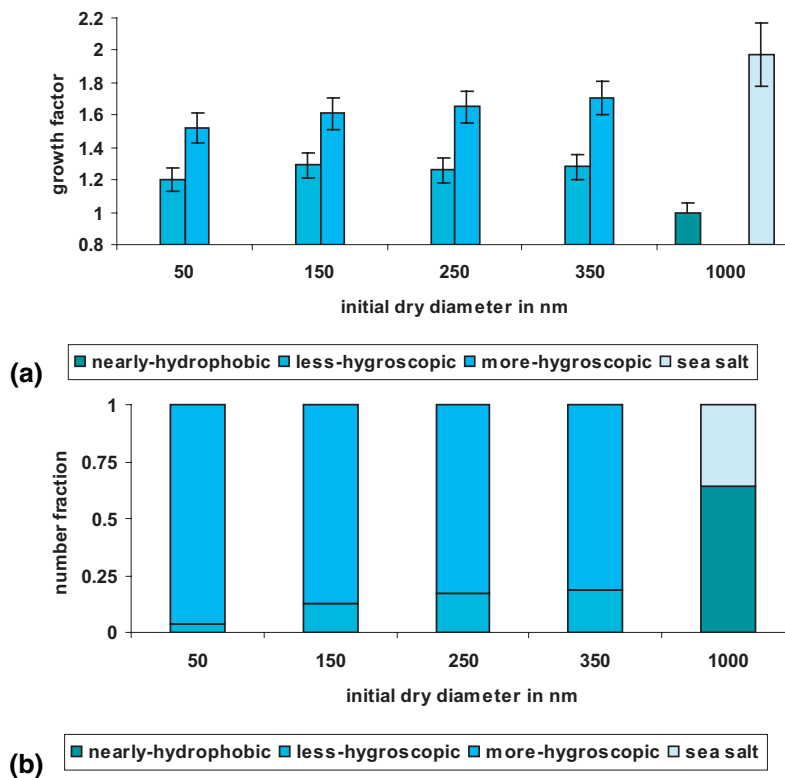
Fig. 5. (a) Hygroscopic growth factors and (b) number fractions for particles with initial dry sizes D_p=50, 150, 250, 350 nm and 1 \mu\text{m} measured at 90% RH for period 3 in an air mass with pollution sources from Japan.
