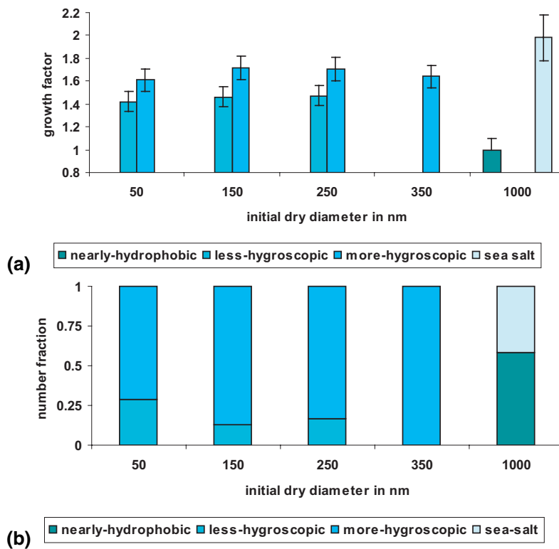
Fig. 4. (a) Hygroscopic growth factors and (b) number fractions for particles with initial dry sizes D_p=50, 150, 250, 350 nm and 1 \mu\text{m} measured at 90% RH for period 2 in an air mass with pollution sources from Korea/Japan .
