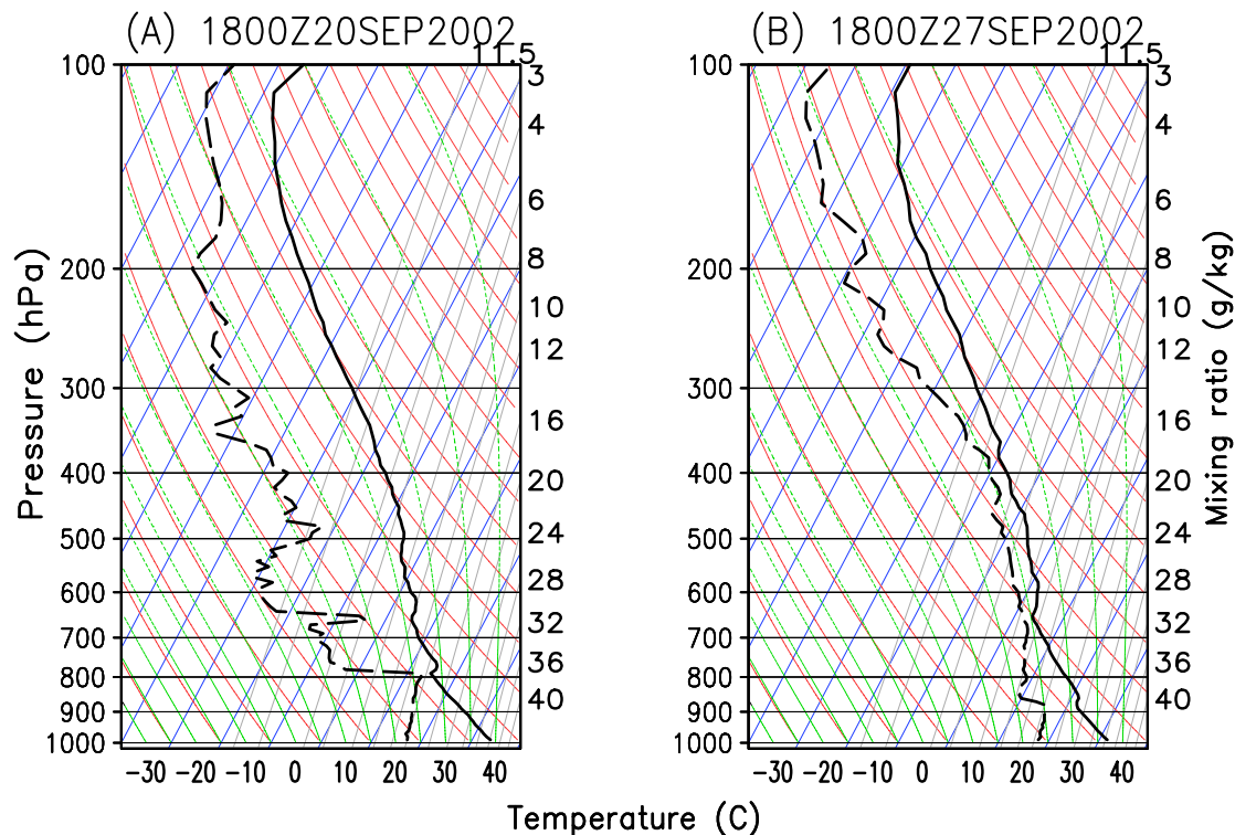
Fig. 2. Temperature (solid) and dew point temperature (dashed) profiles from radiosondes launched in Rondonia ( 11^{\circ}\text{S} , 60^{\circ}\text{W} ) shown as skew T – log p diagrams. Case (a) depicts the condition around 18:00 Z on 20 September 2002, classified as the “dry” case. (b) is the “wet” case corresponding to around 18:00 Z on 27 September 2002.
