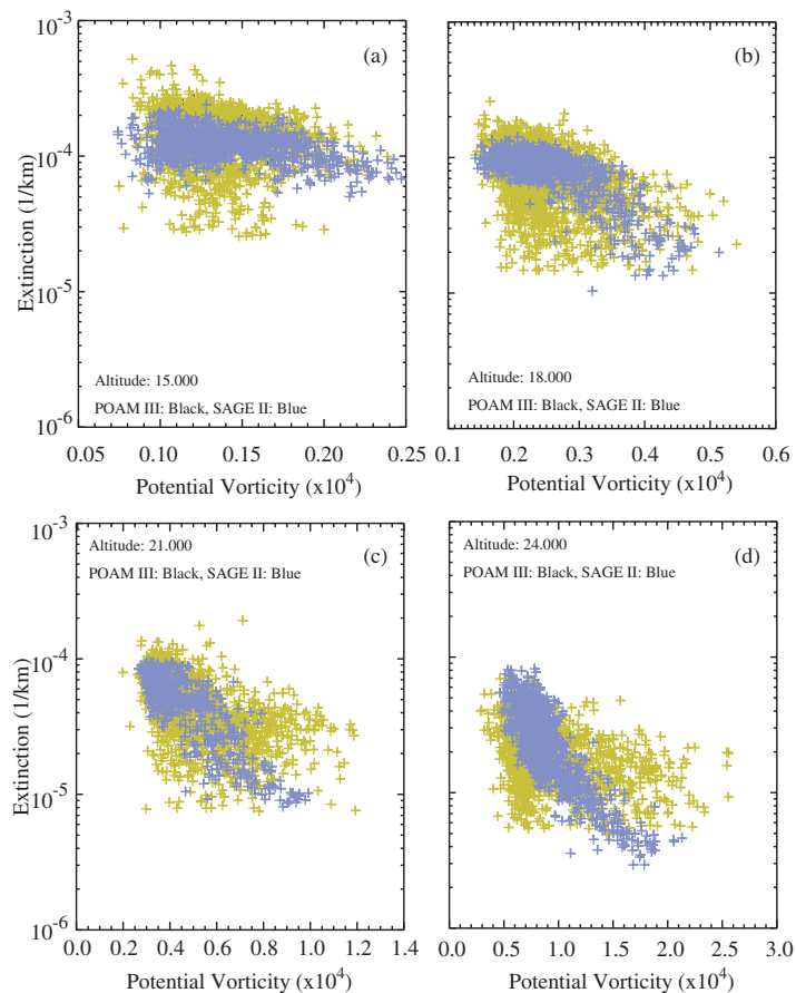
Fig. 6. This figure shows the distribution of 1020-nm aerosol extinction coefficient measured by POAM III (gold) and SAGE II (blue) at 15 (a) , 18 (b) , 21 (c) , and 24 km (d) for January through March of 2003 through 2005. The plots show all data without any matching requirements.
