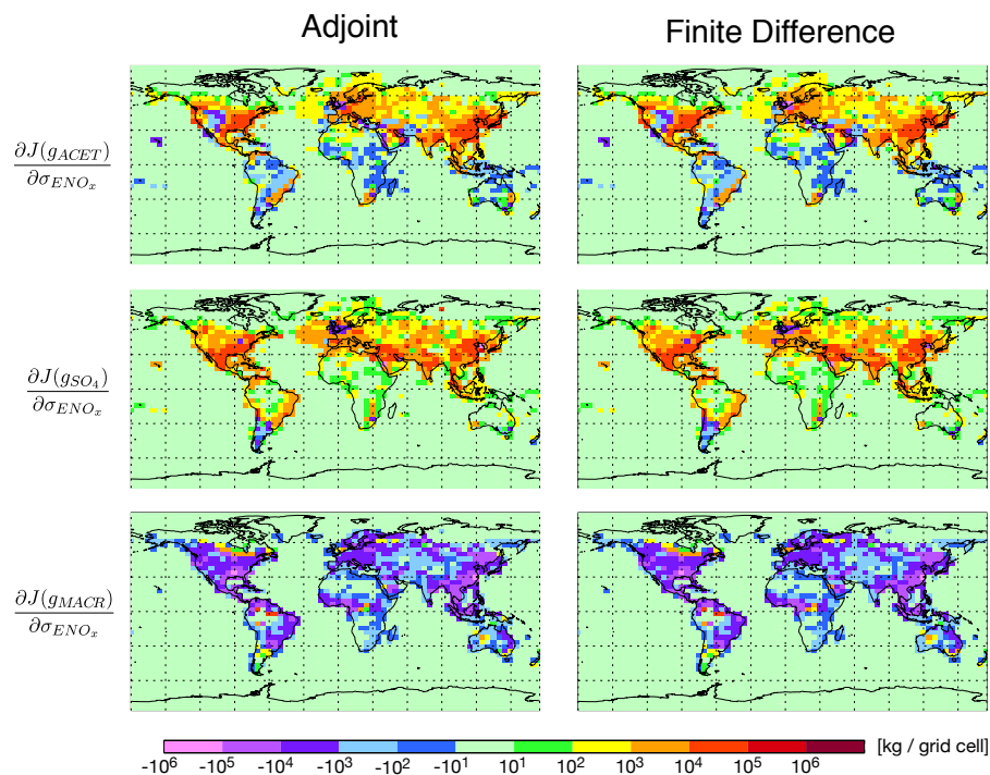
Fig. 2. Chemistry adjoint validation. Full chemistry (only) simulation for 1 week. In the left column are the gradients of the masses of acetone (ACET), sulfate aerosol ( SO_4 ), and methacrolein (MACR) at the surface with respect to anthropogenic emissions of NO_x . In the right column are the same quantities calculated using the finite difference method.
