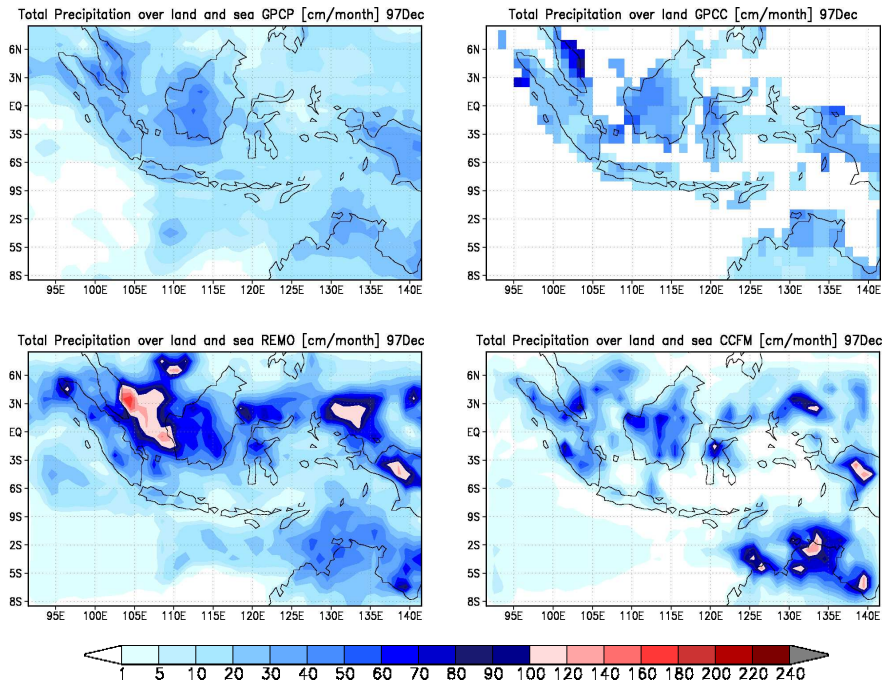
Fig. 10. As Fig. 8, but for December 1997.
