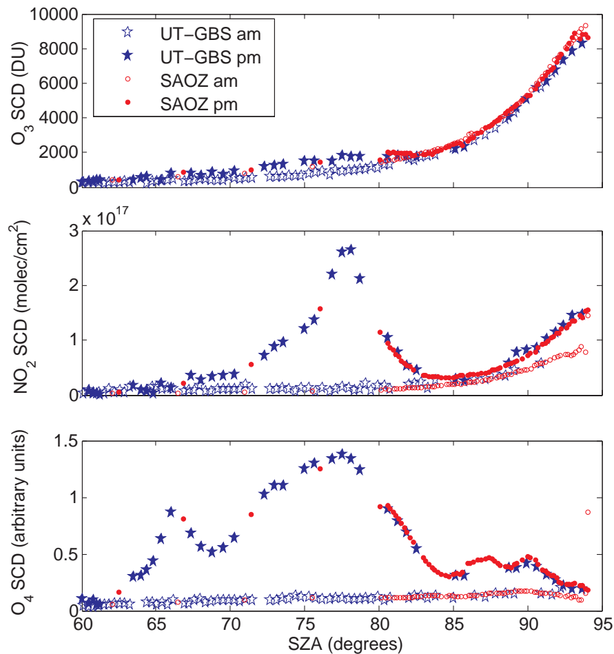
Fig. 5. Ozone, NO 2 , and O 4 slant column densities measured by UT-GBS and SAOZ on 28 August 2004.
