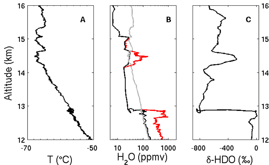
Fig. 3. Profile of (A) temperature, (B) H 2 O mixing ratios (measured vapour: black; saturation vapour with respect to ice: grey; total (vapour plus ice: red) and δ-HDO in a profile obtained on 28 July 2002 over southern Florida. Two isotopically distinct cloud layers are seen: anvil cirrus outflow from convection located below 13 km altitude, and a more tenuously clouded TTL layer centered at 14.5 km altitude. Values of δ-HDO in the anvil indicate it originated from lower tropospheric air. In the TTL cloud, values of δ-HDO and H 2 O are intermediate to those in the anvil and TTL. The implication is that the TTC formed from a mixing process between surface and TTL air masses.
