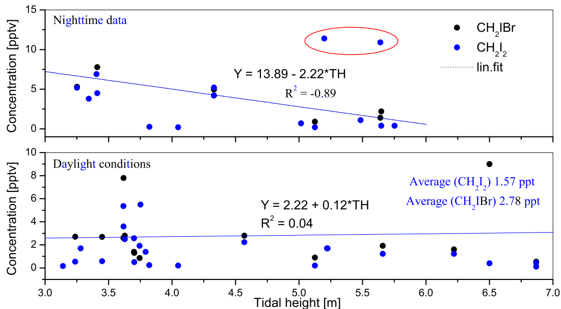
Fig. 9. Concentration of the short lived iodocarbons CH 2 I 2 and CH 2 IBr in the absence (upper panel) and in the presence (lower panel) of sunlight during 2003 Brittany campaign. At night the observed concentration of the iodocarbons significantly decreases with increasing water level.
