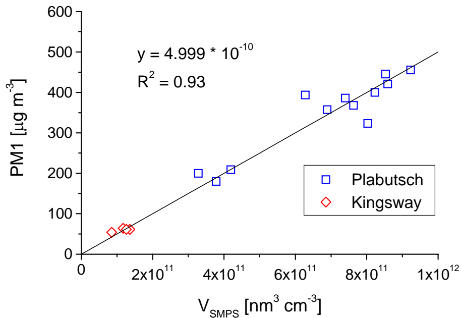
Fig. 8. Correlation between the SMPS particle volume ( V_{SMPS} ) and PM1 (filter sampling).
