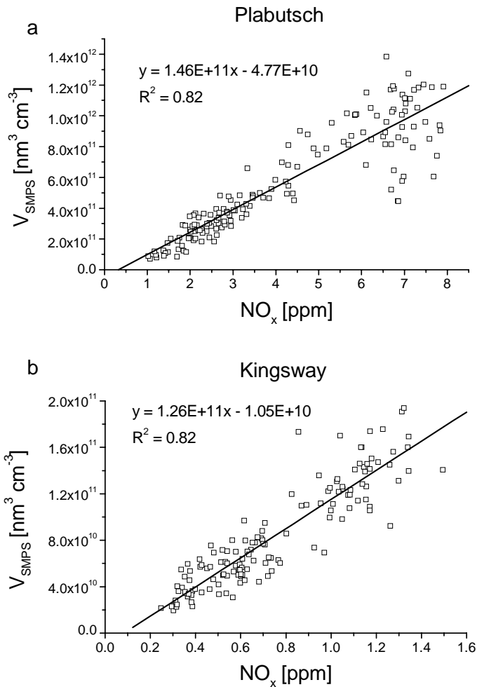
Fig. 7. Correlation between NO x and the particle volume ( V_{SMPs} ) in the Plabutsch (a) and the Kingsway (b) tunnel.
