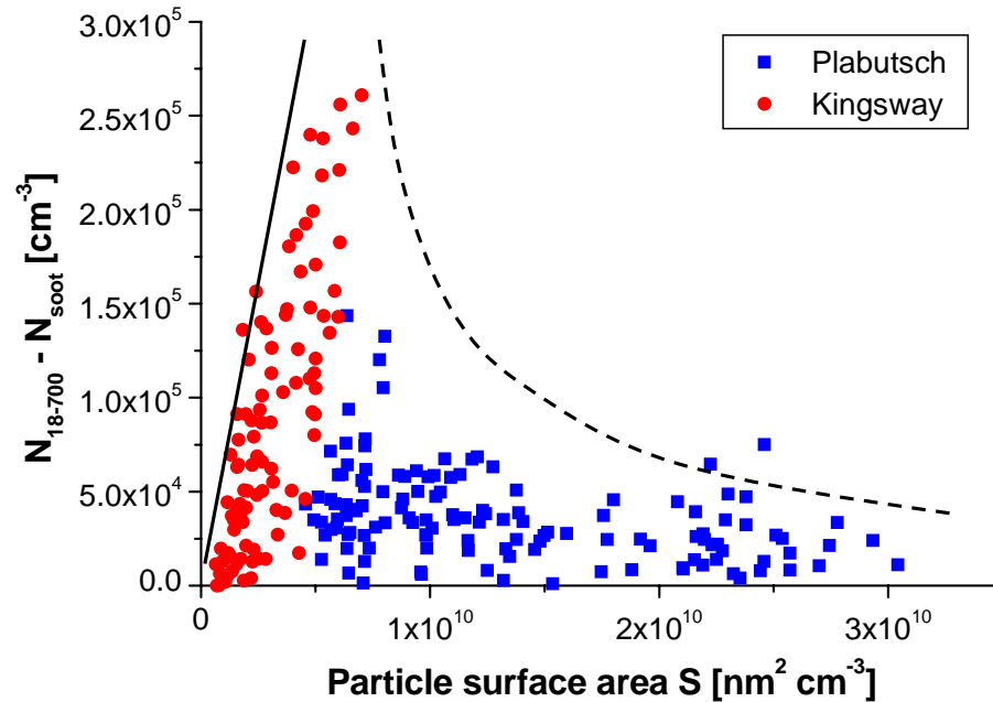
Fig. 6. Scatter plot of the aerosol surface area concentration versus the number concentration of particles in the size range D=18-700 nm subtracted by the number concentration of the soot particles ( N_{18-700}-N_{soot} ) observed in the two tunnels.
