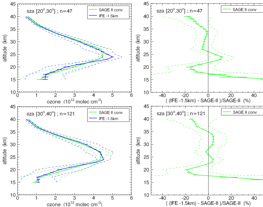
Fig. 6. Shown here are comparisons between IFE1.61 and SAGE II, convolved with the IFE averaging kernels, grouped into 10 degree solar zenith angle bands (which are shown on top of the plots). The number of collocations 'n' are indicated in each plot.
