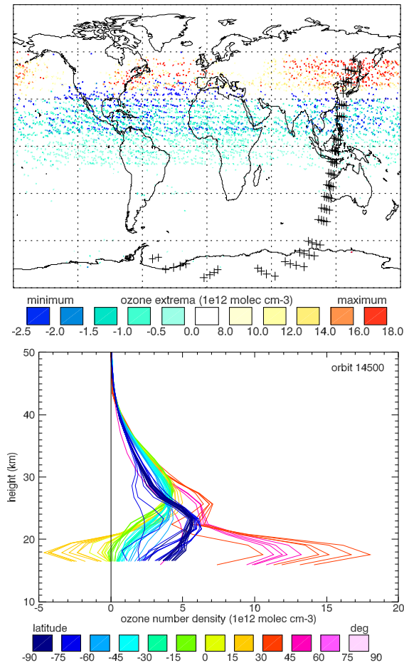
Fig. 9. Most extreme ozone concentration retrieved per profile, as a function of location (top panel). Of the overplotted orbit (black crosses), all ozone profiles are shown in the bottom panel, where colour indicates their latitude.
