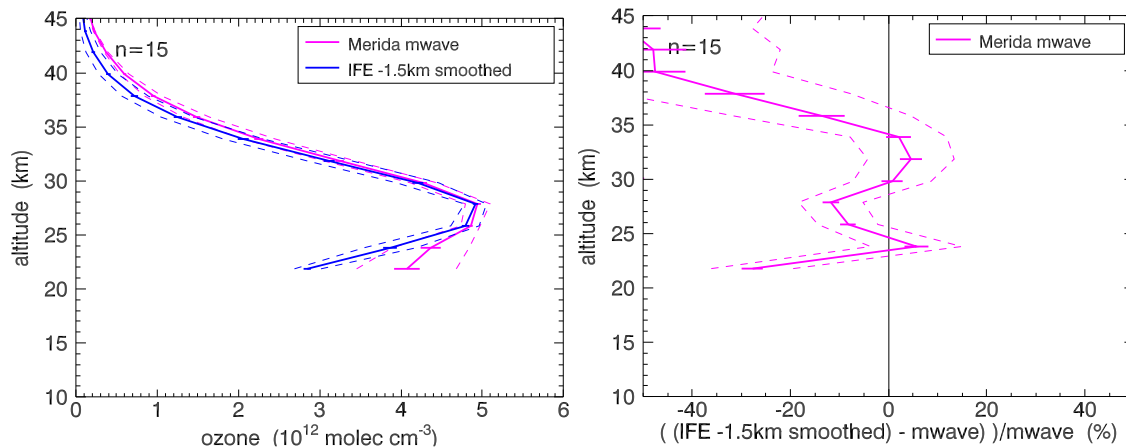
Fig. 8. As Fig. 3, but now with respect to microwave, only for the Merida (Venezuela) location, 15 collocations. ‘Unsmoothed data’ refer to comparison between original IFE and microwave results, ‘smoothed data’ refer to a comparison where IFE data were smoothed using the microwave radiometer averaging kernels.
