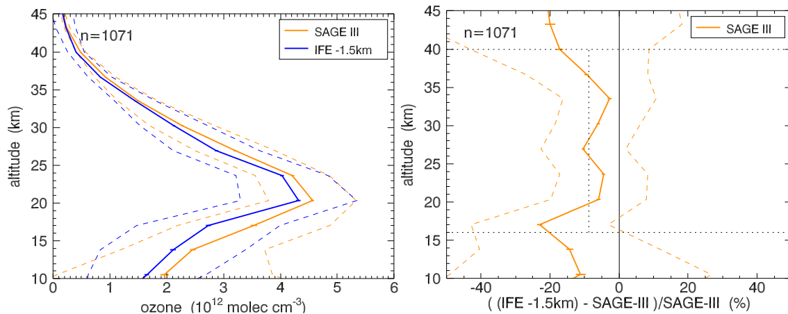
Fig. 5. As Fig. 4, but now with respect to SAGE III (1071 collocations).
