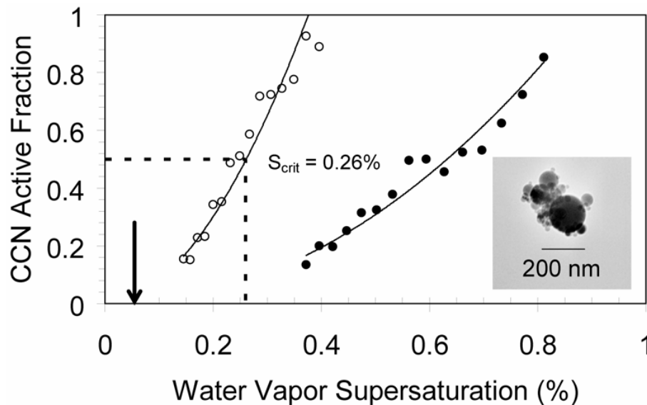
Fig. 2. Measured CCN activity for 200 nm alumina-silicate particles. Symbols indicate cases of untreated particles (closed circles) and particles treated with \text{H}_2\text{SO}_4 (open circles). The lines indicate exponential fits to the data, and S_{\text{crit}} is the point on the line where 50% of the particles have activated as CCN. The critical supersaturation of a 200 nm pure sulfuric acid solution particle is indicated by the arrow. The insert shows a TEM image of a treated 200 nm core-sized alumina-silicate particle.
