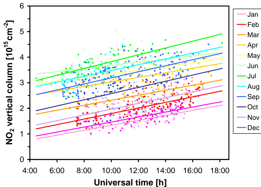
Fig. 3. The Zugspitze FTIR NO 2 -vertical column data set as shown in Fig. 2, but plotted as a function of the time of the day. Data were classified into 12 months and linear fits to the diurnal increase performed on the monthly data sets.
