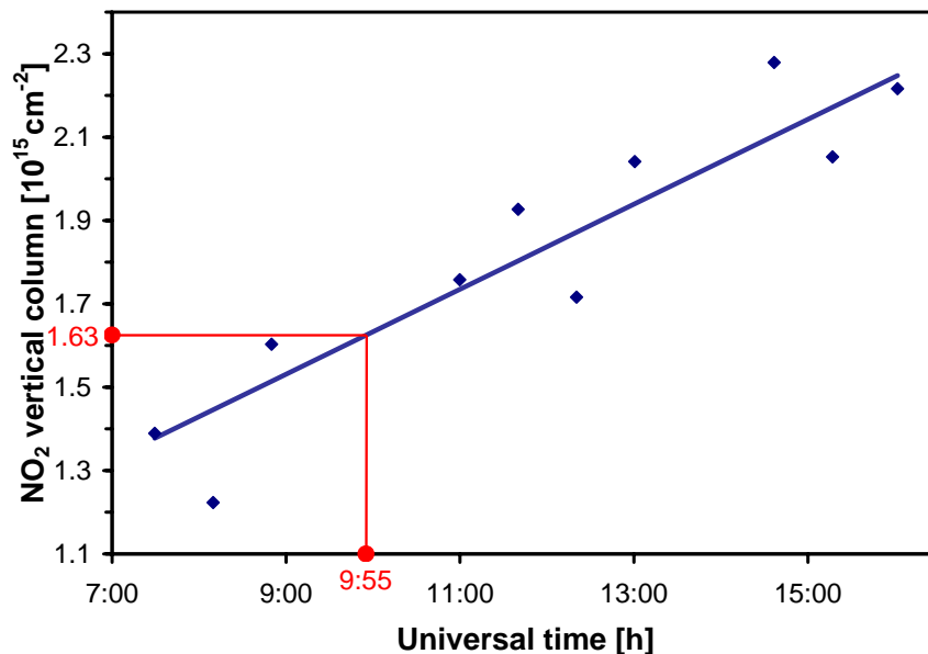
Fig. 4. Zugspitze FTIR NO 2 vertical column data – individual measurements of one arbitrarily chosen day. The blue line is a fit with a constant slope (i.e., the daytime increasing rate of 1.02\text{E}+14\text{ cm}^{-2}/\text{h} ) with only the offset as fit parameter. The red lines illustrate the concept of the “virtual-coincidence column”, here for a 09:55 UT satellite overpass. For details, see text.
