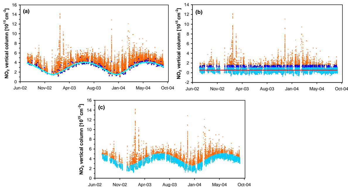
Fig. 6. Orange points: the SCIAMACHY NO 2 vertical column data set analyzed with the UB1.5 DOAS algorithm developed at the University of Bremen. Plotted are columns retrieved from individual measurements within a 200-km selection radius around the Zugspitze. The 3 steps of the pollution clearing for SCIAMACHY data in a 200-km radius around Zugspitze are: (a) Fit (blue line) to minimum values (marine). (b) Substraction of the fit function result (orange); data cut off at 2 times the average columns value of orange points (marine); one iteration (bright blue) based on average value of marine points (red line). (c) Adding of the fit function result from (a) yields final pollution corrected data (bright blue).
