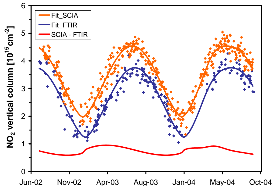
Fig. 7. Blue: The Zugspitze FTIR NO 2 -vertical column data set as in Fig. 2, but now the daily virtual-coincidence columns for the time of ENVISAT overpass are plotted. Orange: SCIAMACHY NO 2 -vertical column data, i.e., daily averages of the pollution-cleared data (see Fig. 6c) are plotted. Red: Difference between orange and blue line. Mathematical details of the analytic function that has been fitted to both data sets (solid lines) are described in Appendix A.
