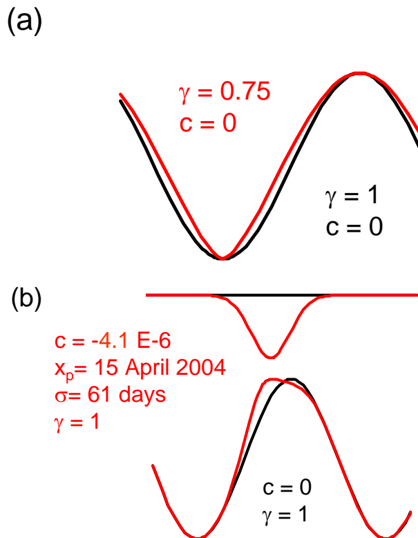
Fig. A1. Schematics to illustrate the analytic function used to fit the annual cycle of NO 2 columns, i.e., its deviations from a sine function. (a) Decrease of the radius of curvature around the minimum by using \gamma ( <1 ) as a fitting parameter. (b) Shift of maximum to earlier times by a local Gaussian frequency modulation using as fit parameters the strength c , the position in time x_p , and the width \sigma .
