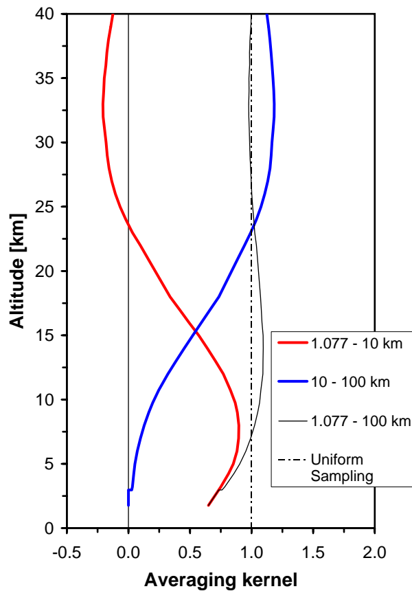
Fig. 11. Averaging kernels for the combined FTIR and SCIAMACHY retrieval of NO 2 , calculated for a solar zenith angle of 20°. Red line: Tropospheric partial column averaging kernel (calculated for 1.077–10 km). Blue line: Stratospheric partial column averaging kernel (calculated for 10–100 km). Black line: total column averaging kernel for the combined retrieval.
