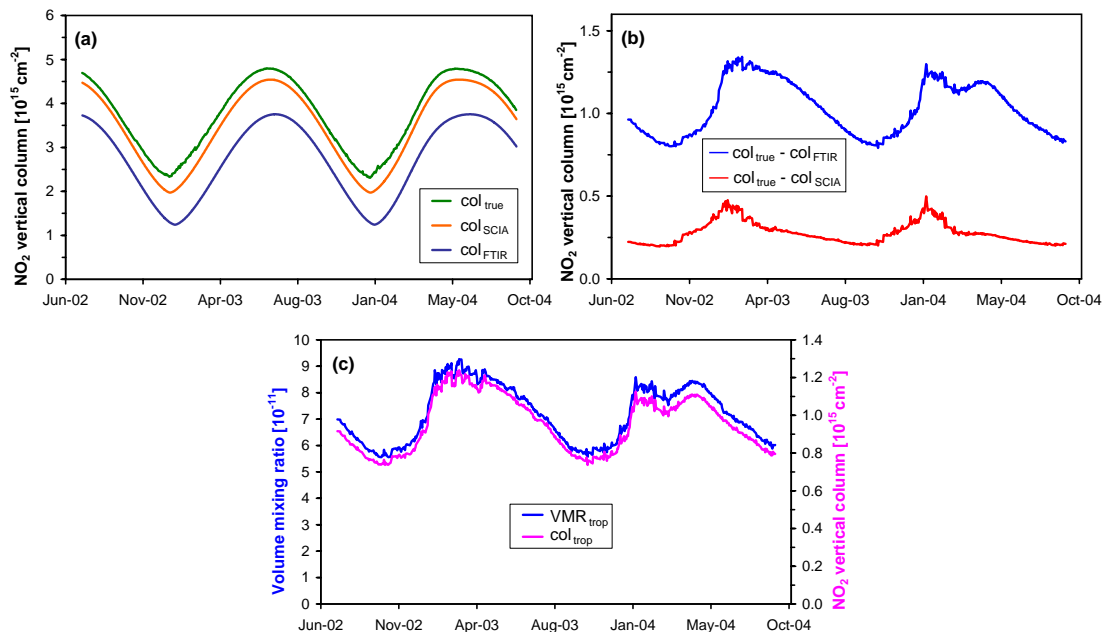
Fig. 12. (a) True column series col_{true} (green) inferred from matching FTIR and SCIAMACHY retrievals. Column series retrieved by SCIAMACHY col_{SCIA} (orange, same as in Fig. 7) and the column series retrieved by FTIR col_{FTIR} (blue, same as in Fig. 7). (b) Difference that has to be added to FTIR and SCIAMACHY, respectively, in order to compensate for the underestimation of the true column by the averaging kernels. (c) Time series of the clean background tropospheric mixing ratio VMR_{trop} obtained from the combined retrieval of FTIR and SCIAMACHY (blue), and the corresponding clean background tropospheric column between 1.077 km–10 km (magenta).
