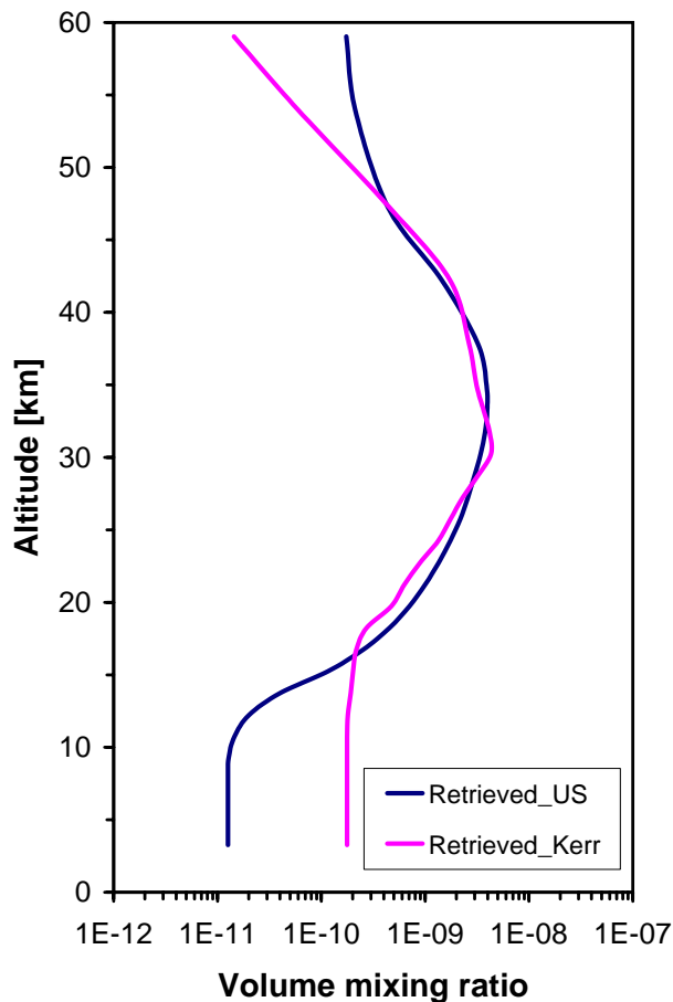
Fig. 1. NO 2 FTIR (profile scaling) retrieval results from one arbitrarily chosen measured spectrum with SZA=61^\circ using two different NO 2 a priori VMR profiles, i.e., the 1976 US Standard atmosphere (blue) versus the retrieval based upon the standard profile by “Kerr et al.” (Rinsland, personal communication, 1999), distributed with the “refmod99” data set (magenta).
