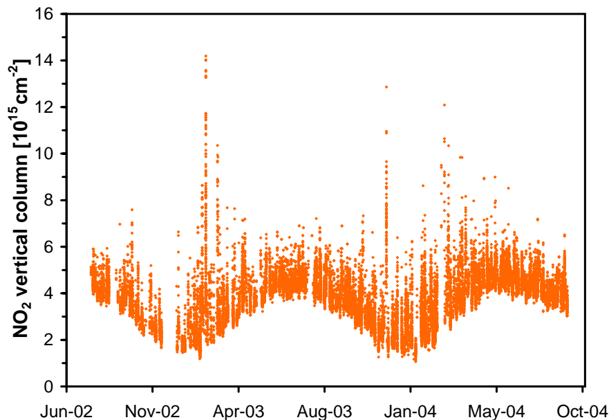
Fig. 5. The SCIAMACHY NO 2 vertical column data set analyzed with the UB1.5 DOAS algorithm developed at the University of Bremen. Plotted are columns retrieved from individual measurements within a 200-km selection radius around the Zugspitze. The US 1976 Standard NO 2 VMR profile with the tropospheric part (<10 km) set to zero was used for air mass factor calculations, assuming no aerosols and a surface albedo of 5%.
