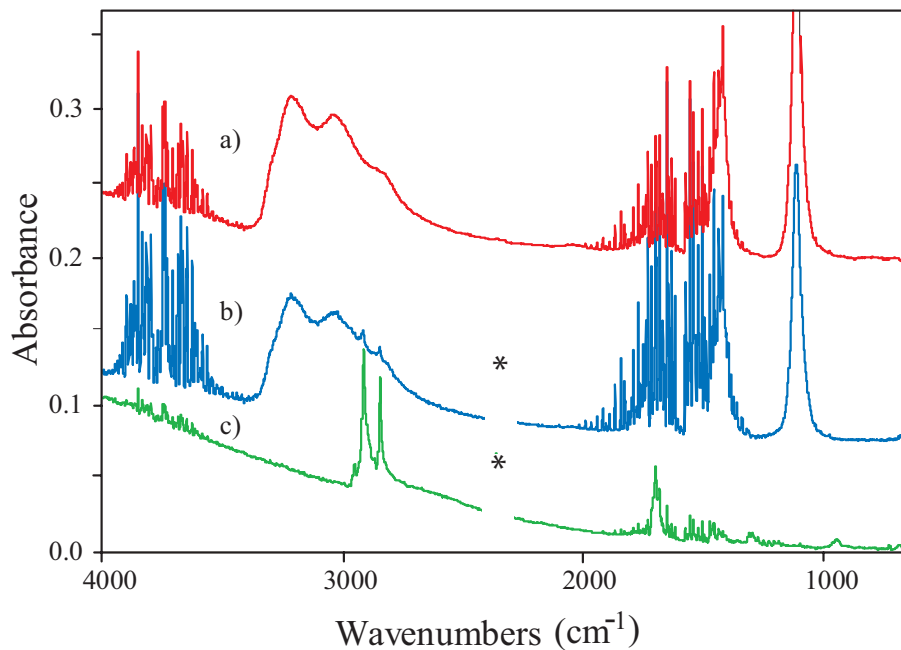
Fig. 2. Representative IR spectra of a) pure ammonium sulfate; b) 48.8 wt% palmitic acid/51.2 wt% ammonium sulfate and c) pure palmitic acid; * indicates CO 2 absorption bands subtracted out; the bands are an artifact from the coating method.
