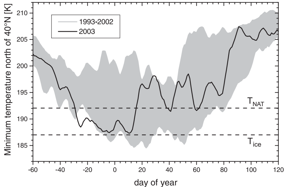
Fig. 2. Minimum temperatures north of 40^\circ\text{N} at the 475 K isentropic level (ECMWF-data). The shaded area depicts the variability for the winters 1992/1993–2001/2002. The dashed lines depict PSC formation temperatures for T_{\text{NAT}} and T_{\text{ICE}} .
