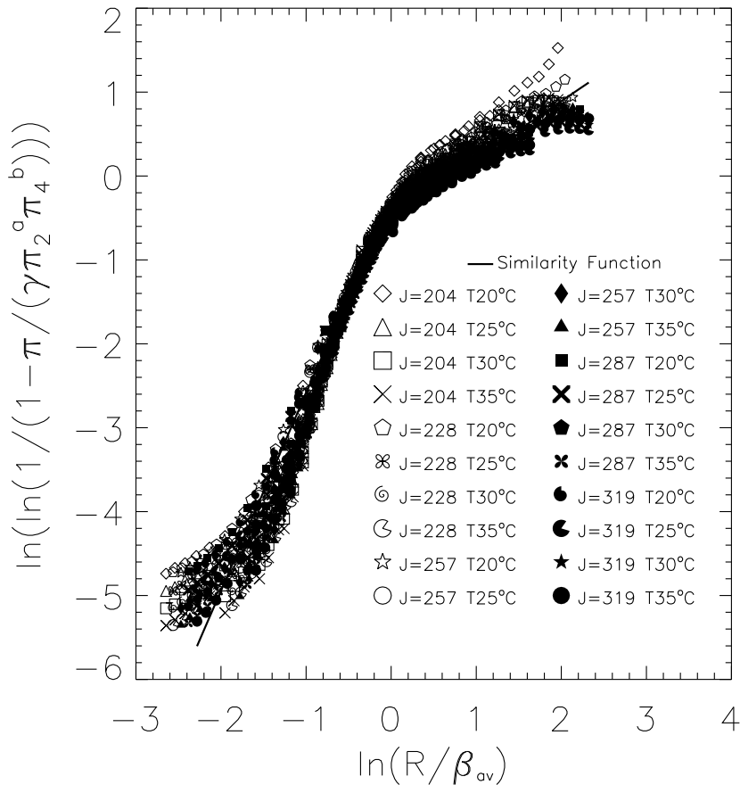
Fig. 5. Weibull transformed model output for RADM2 simulations having five different levels of actinic flux and four different temperatures after horizontal translation by \ln\beta_{av} . Solid lines is the “universal” similarity function.
