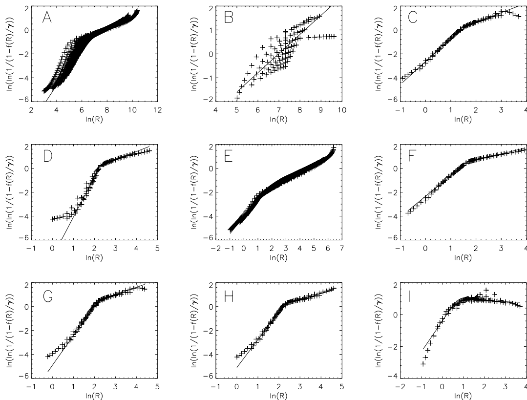
Fig. 4. Weibull transformed similarity relationships for RADM2 classes: (A) ETH (B) HC5 (C) TOLU (D) OLI (E) HCHO (F) ALD. An urban VOC mixture is simulated using (G) the RADM2 mechanism and (H) CB-IV mechanism. Finally, results from MCM using propene are given in (I) . In each plot model output is given by “+” signs and the similarity function by solid lines.
