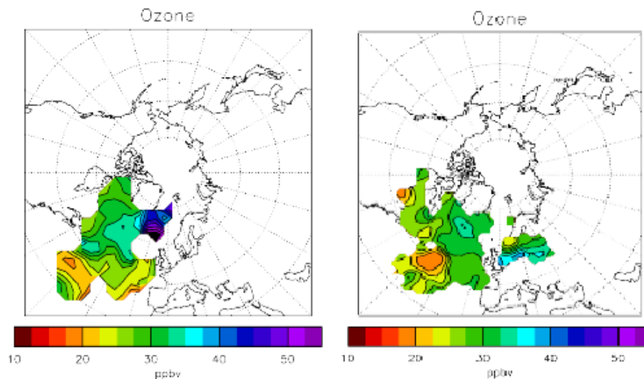
Fig. 24. Map of origin-averaged ozone. Plots showing average ozone data (DEFRA) for every hour during EASE96 on left and NAMBLEX on right which are used to label the origin of the 5 day back trajectory from Mace Head.
