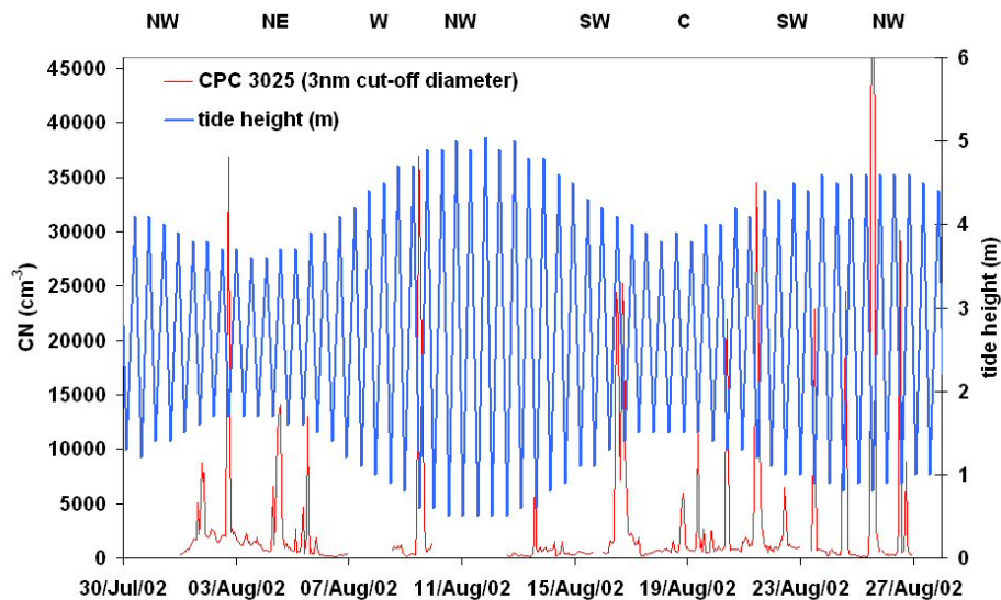
Fig. 17. Time-series of CN >3 nm diameter and tidal height for the NAMBLEX campaign.
