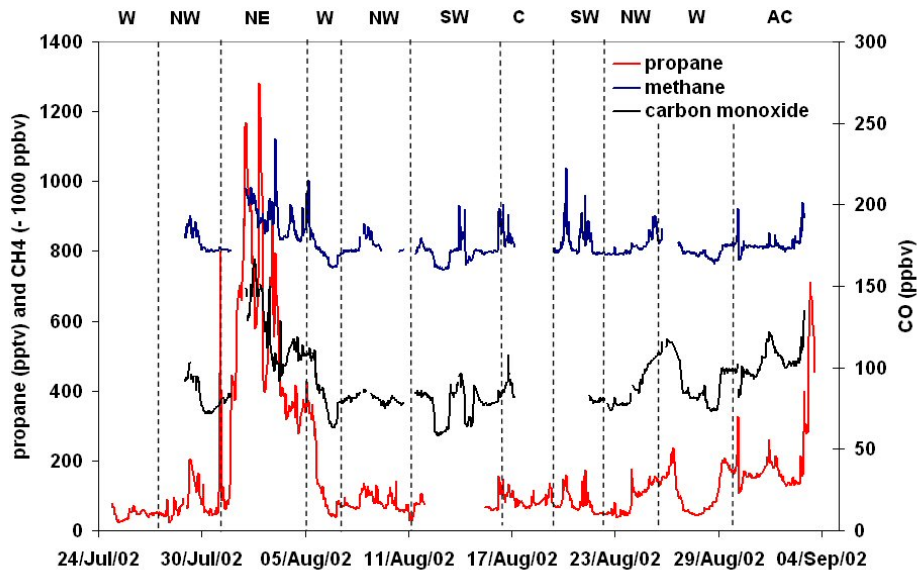
Fig. 10. Time-series of methane, propane and carbon monoxide.
