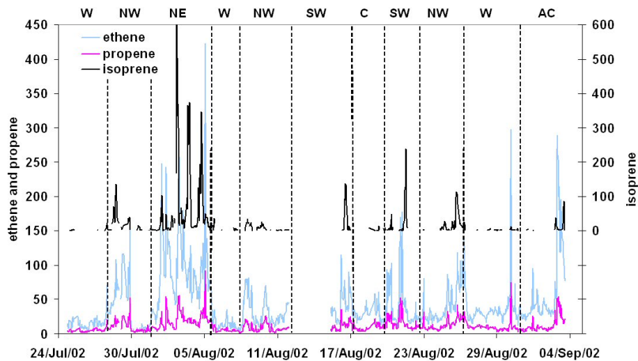
Fig. 11. Time-series of ethene, propene, and isoprene (vertically displaced for clarity).
