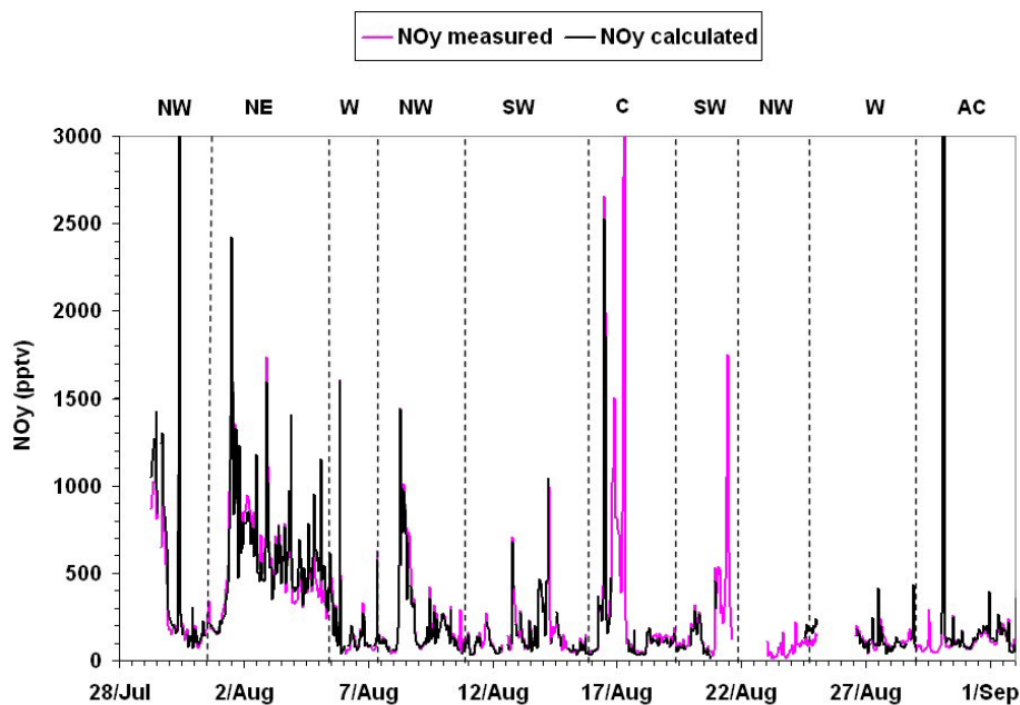
Fig. 13. Time-series of measured and calculated \text{NO}_y , the latter by summing the measured \text{NO} , \text{NO}_2 , \text{HNO}_3 , PAN and organic N.
