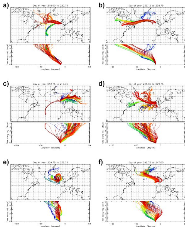
Fig. 20. Trajectories illustrating air flow during some periods of the 6 classifications. In all panels the colours correspond to time during the period (every hour) moving through the rainbow from blue to red. The classifications are based on the final day of the trajectories: (a) 00:00 UT 6 August–18:00 UT 8 August (Second W period), (b) 12:00 UT 24 August–18:00 UT 26 August (Third NW period), (c) 18:00 UT 31 August–00:00 UT 6 August (NE period), (d) 12:00 UT 12 August–18:00 UT 17 August (First SW period), (e) 18:00 UT 17 August–18:00 UT 20 August (Cyclonic period) (f) 18:00 UT 30 August–00:00 UT 4 September (Anti-cyclonic period).
