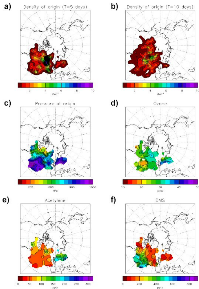
Fig. 19. (a): Density of origin plot for 5-day back trajectories from 500 m above Mace Head during NAMBLEX, (b): As (a) but for 10 days, (c): Origin-averaged pressure at origin of air mass, (d): Origin-averaged ozone, (e): Origin-averaged acetylene, (f): Origin-averaged DMS. (c–f based on 5-day trajectories). 12249
