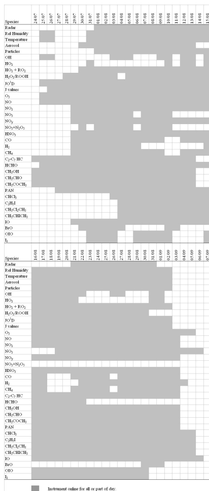
Fig. 5. Time-line showing data coverage for the NAMBLEX campaign, 2002.
