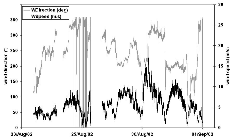
Fig. 3. Time-series of wind direction and wind speed from measurements made from the top of the 10 m tower by NUI, Galway.
