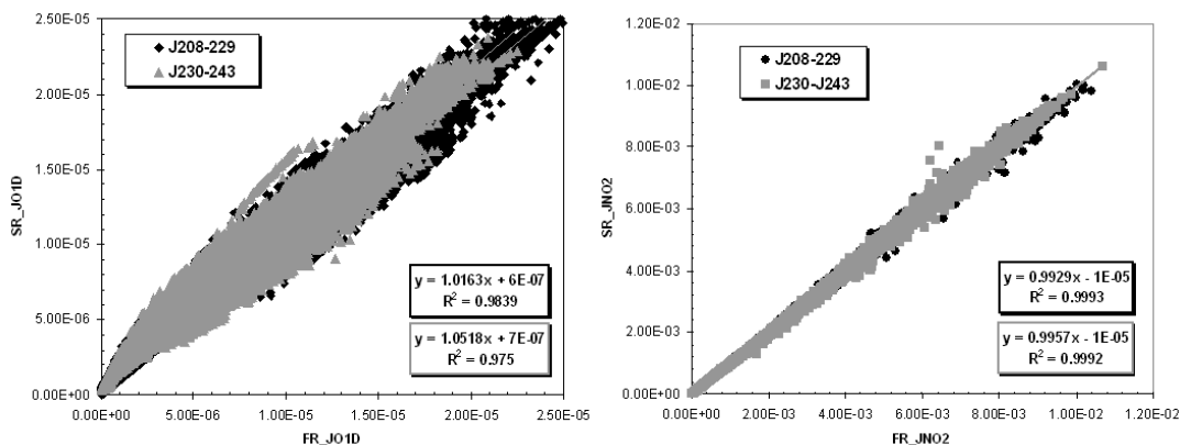
Fig. 15. (a): Correlation plot for j\text{-(O}^1\text{D)} measured using the University of Leicester's filter radiometer (FR) and diode array spectroradiometer (SR). (b): Correlation plot for j\text{-(NO}_2\text{)} measured using the University of Leicester's filter radiometer (FR) and diode array spectroradiometer (SR). The two Julian day ranges refer to data from the first and second halves of the campaign, respectively.
