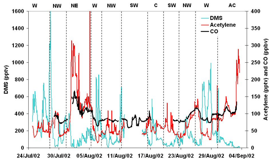
Fig. 8. Time-series of carbon monoxide, acetylene and dimethyl sulfide.
