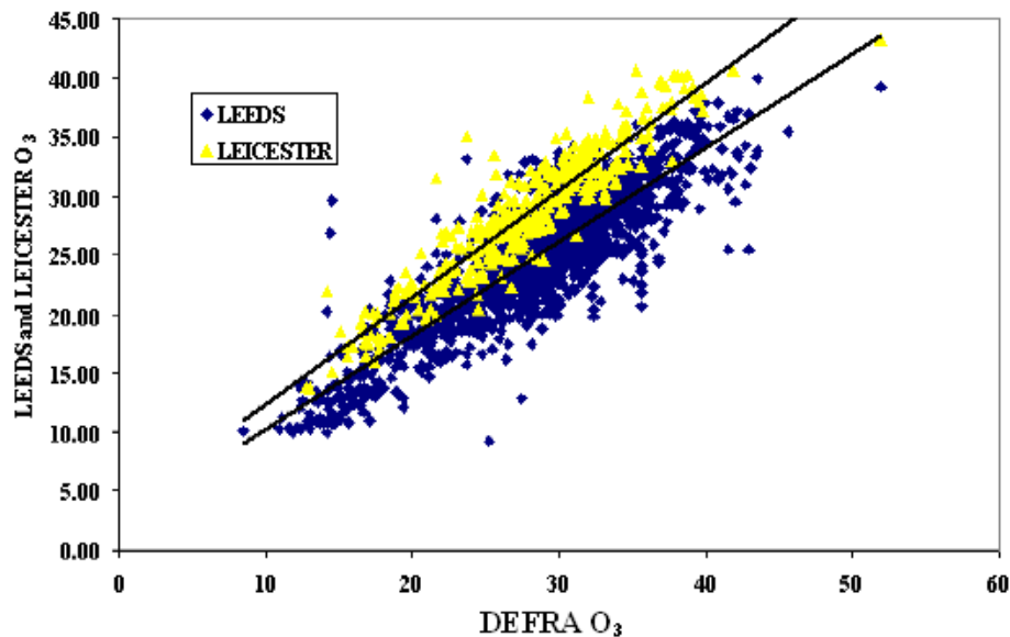
Fig. 7. Correlation of various O 3 measurements made during NAMBLEX at Mace Head for the period 17–20 August and 26 August–4 September 2002.
