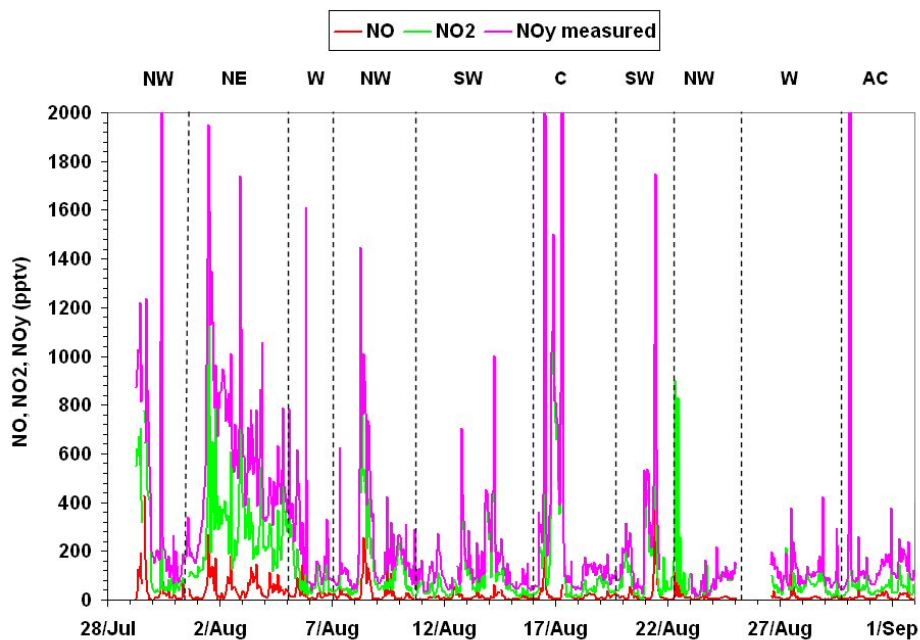
Fig. 12. Time-series of NO, NO 2 , and measured NO y .
