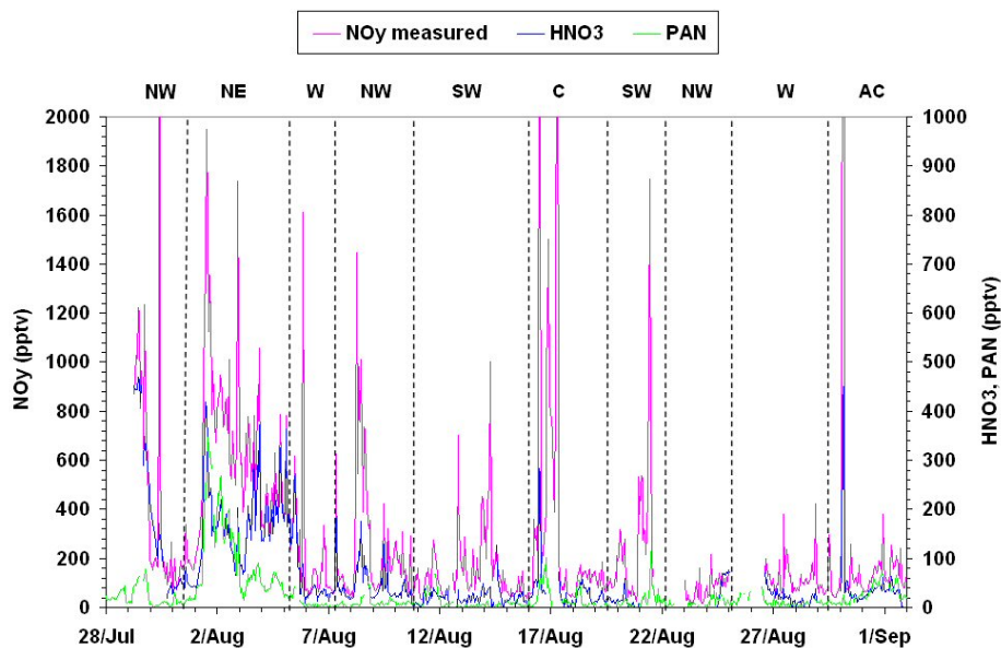
Fig. 14. Time-series of measured \text{NO}_y , \text{HNO}_3 , and PAN.
