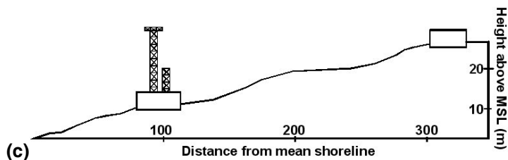
Fig. 1. (a): A map of the Connemara region (Ireland inset) showing the Mace Head site and Croaghnaekeela island where the DOAS retro-mirror was situated. (b): A plan of the site showing the position of the permanent buildings, containers, instruments, sampling towers and sampling points for each measurement, (c): Side view of site.
