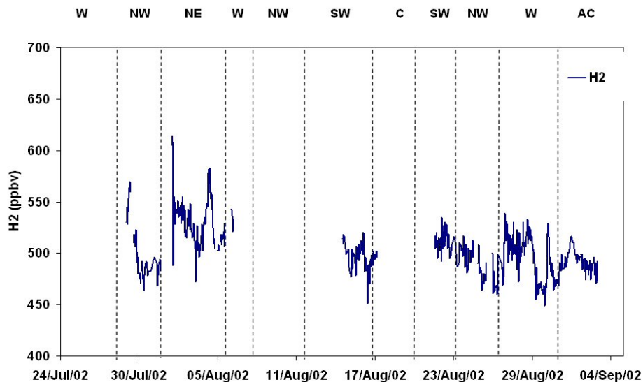
Fig. 9. Time-series for hydrogen at Mace Head during NAMBLEX.
