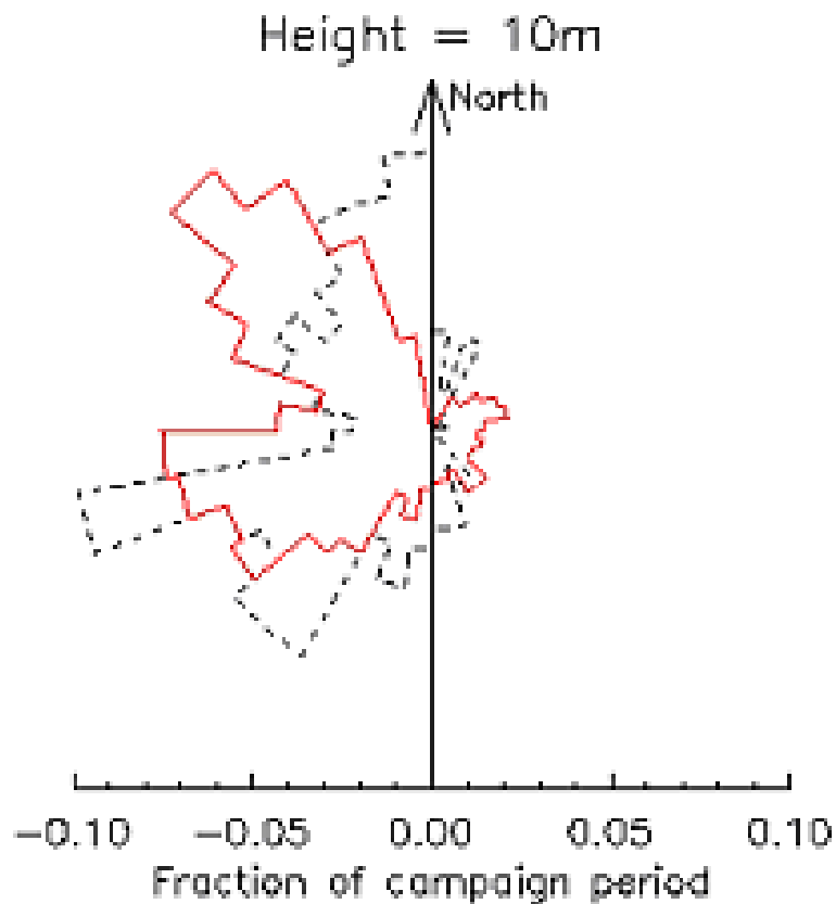
Fig. 18. Wind Rose showing the frequency of different wind directions for the local measurement from the met mast (red) and for the ECMWF analyses at 10 m (dashed).
