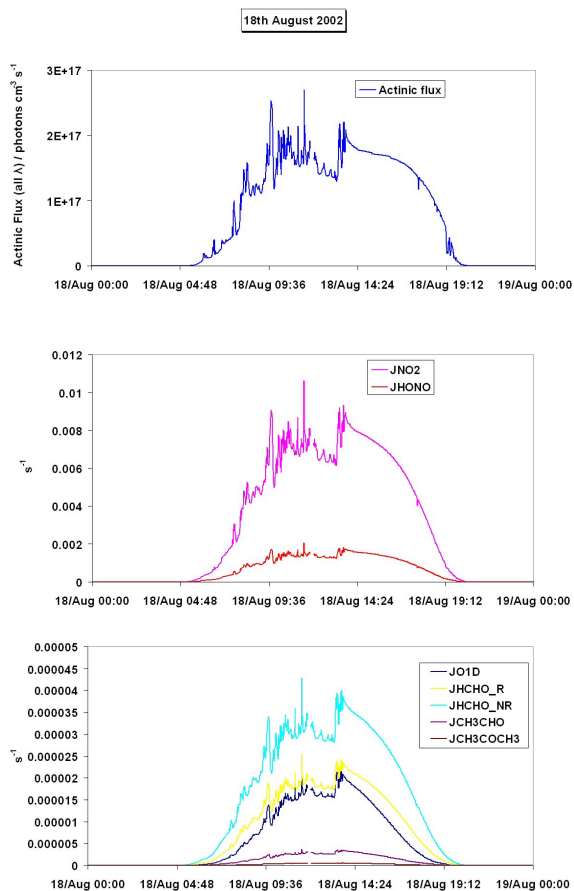
Fig. 16. (a): Actinic flux, (b): j(\text{NO}_2) and j(\text{HONO}) , (c): j(\text{O}_1\text{D}) , j(\text{HCHO})_{\text{NR}} (non-radical, \text{HCHO} + h\nu \rightarrow \text{H}_2 + \text{CO} ), j(\text{HCHO})_{\text{R}} (radical, \text{HCHO} + h\nu \rightarrow \text{HCO} + \text{H} \rightarrow \text{HO}_2 + \text{HO}_2 + \text{CO} ), j(\text{CH}_3\text{CHO}) , and j(\text{CH}_3\text{COCH}_3) for a clean day 18 August 2002.
