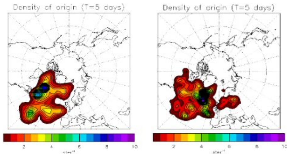
Fig. 22. Density of origin plots using 5-day back trajectories for EASE96 (left) and NAMBLEX (right).
