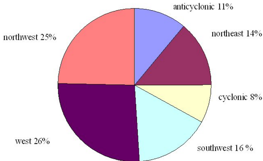
Fig. 21. The distribution of trajectory classifications during NAMBLEX.
