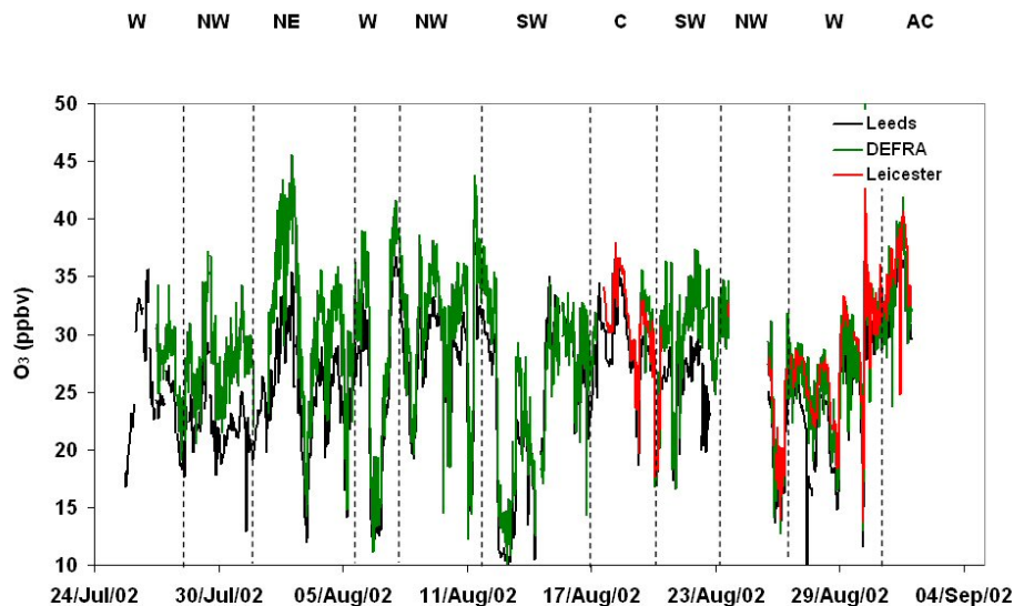
Fig. 6. Time-series of 30-min averaged O_3 .
