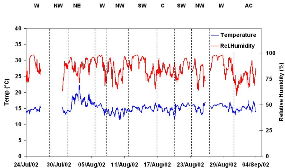
Fig. 4. Time-series of temperature and relative humidity, (annotated lines divide the periods of different air mass origin).
