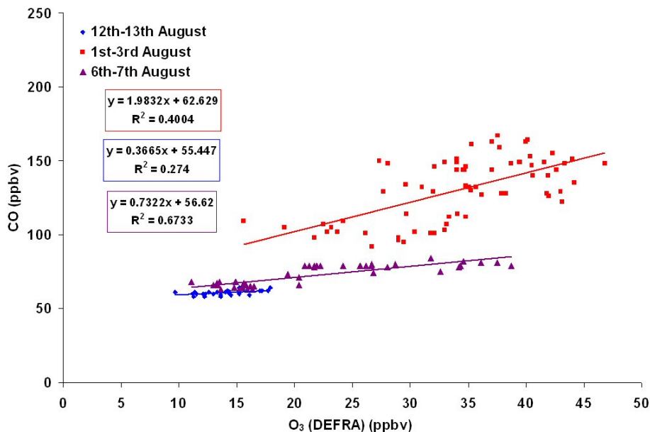
Fig. 23. CO versus O 3 for a “polluted” period (1–3 August in red) a “clean” westerly period (6–7 August in purple), and for a “cleaner” south westerly period (12–13 August in blue) during NAMBLEX 2002.
