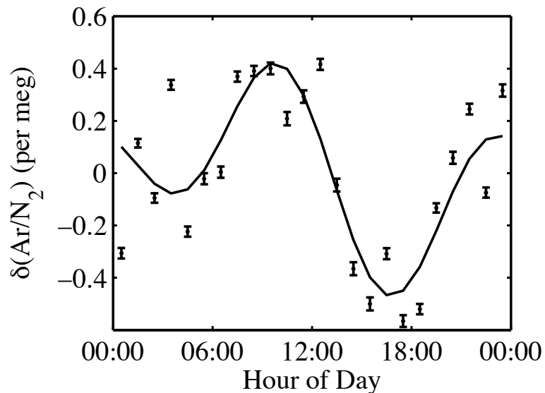
Fig. 5. Average diurnal cycle from semi-continuous data between 1 June 2004 and 31 May 2005. Within this period, we have 75 days in which we have 24 hourly determinations. We remove the daily mean and then average all 75 points for each hour of the day.
