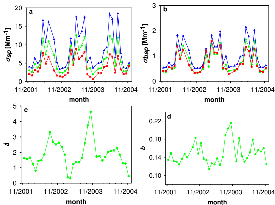
Fig. 3. Monthly average values of (a) \sigma_{sp} at three wavelengths, (b) \sigma_{bsp} at three wavelengths, (c) \hat{a} and (d) b at 550 nm. Triangles, circles and squares correspond to \sigma_{sp} and \sigma_{bsp} values at 450 nm, 550 nm and 700 nm, respectively.
