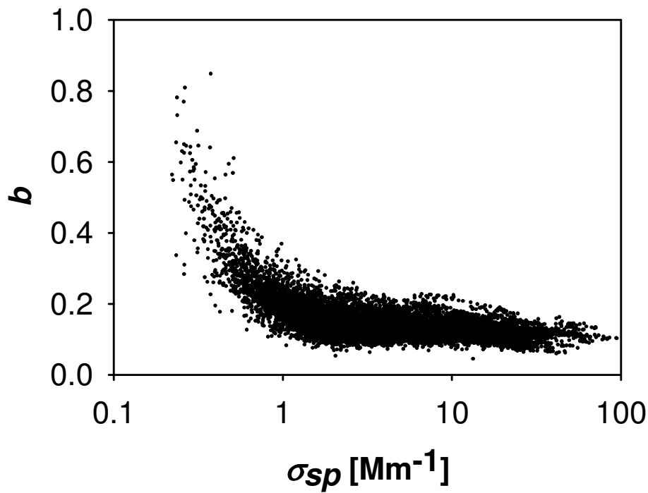
Fig. 4. Relation between \sigma_{sp} and b at 550 nm.
