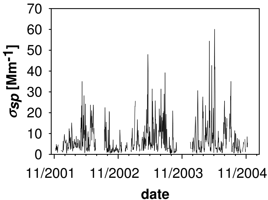
Fig. 2. Time-series of \sigma_{sp} at 550 nm.
