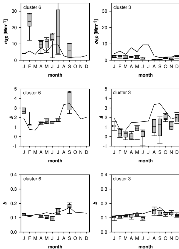
Fig. 9. Box whisker diagrams of the monthly variation of \sigma_{sp} at 550 nm (top), \hat{a} (middle) and b at 550 nm (bottom) for clusters 6 and 3. The box has a horizontal line at the lower quartile, median and upper quartile values. The whiskers are lines extending from each end of the box to show the 10th and 90th percentiles. The curve shows the median value of all data, regardless of transport pattern.
