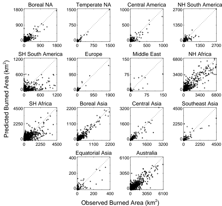
Fig. 10. Scatter plots of burned area predicted by regional regression trees vs. “true” burned area derived from 500-m burned area maps. Axes show area in km 2 .
