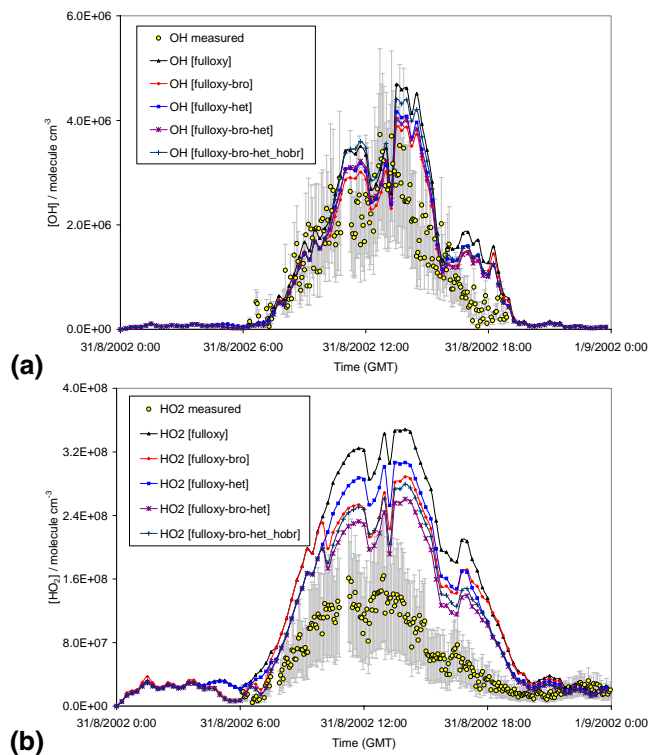
Fig. 7. Model-measurement comparison with the improved models (31 August). (a) OH, (b) HO 2 . The measurements 2 \sigma standard deviation is shown in grey.
