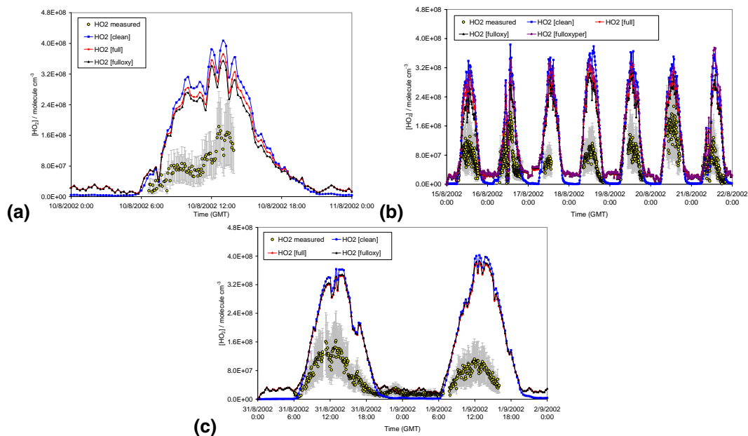
Fig. 3. Model-measurement comparison for HO 2 with the base models. (a) 10 August, (b) 15–21 August, (c) 31 August–1 September. The measurements 2σ standard deviation is shown in grey.
