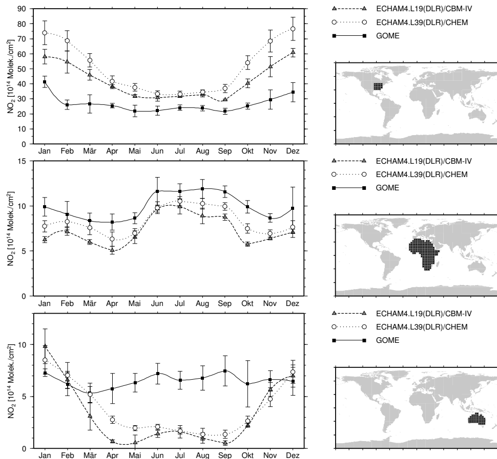
Fig. 3. Regional tropospheric NO 2 -columns derived from GOME satellite data (Richter and Burrows, 2002) and ECHAM4 model simulations (in 10 14 mol. cm -2 ). The respective geographic region for averaging is indicated in black: eastern USA, Africa and Australia.
