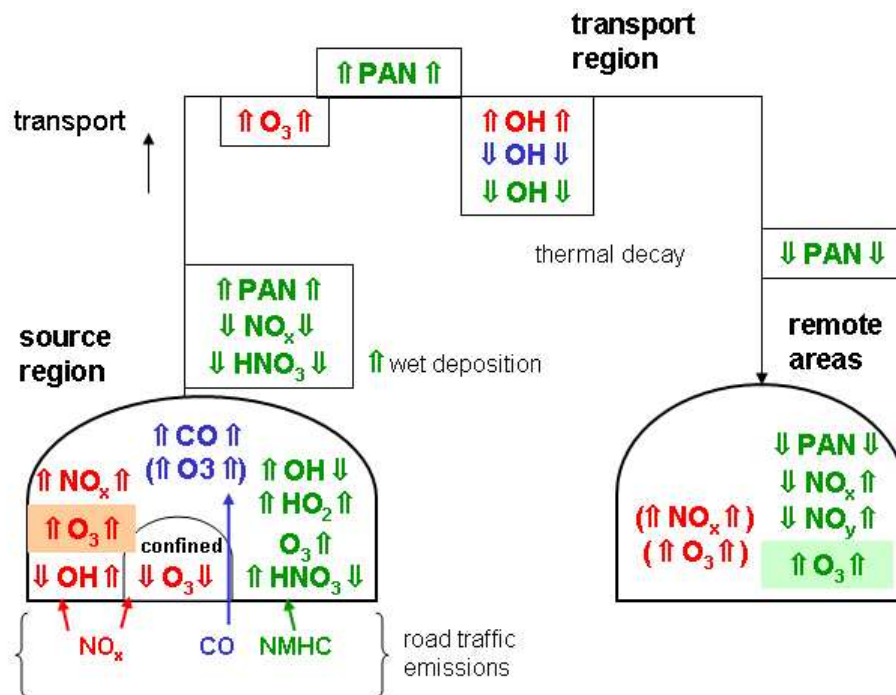
Fig. 8. Scheme illustrating the impact of individual components of road traffic emissions on atmospheric composition: NO x (red), CO (blue), NMHCs (green). An arrow up indicates increase, down a decrease; the arrows on the left of the specie describe the change in winter, those on the right the change in summer. Weak processes are in parenthesis, major processes are highlighted with a coloured background.
