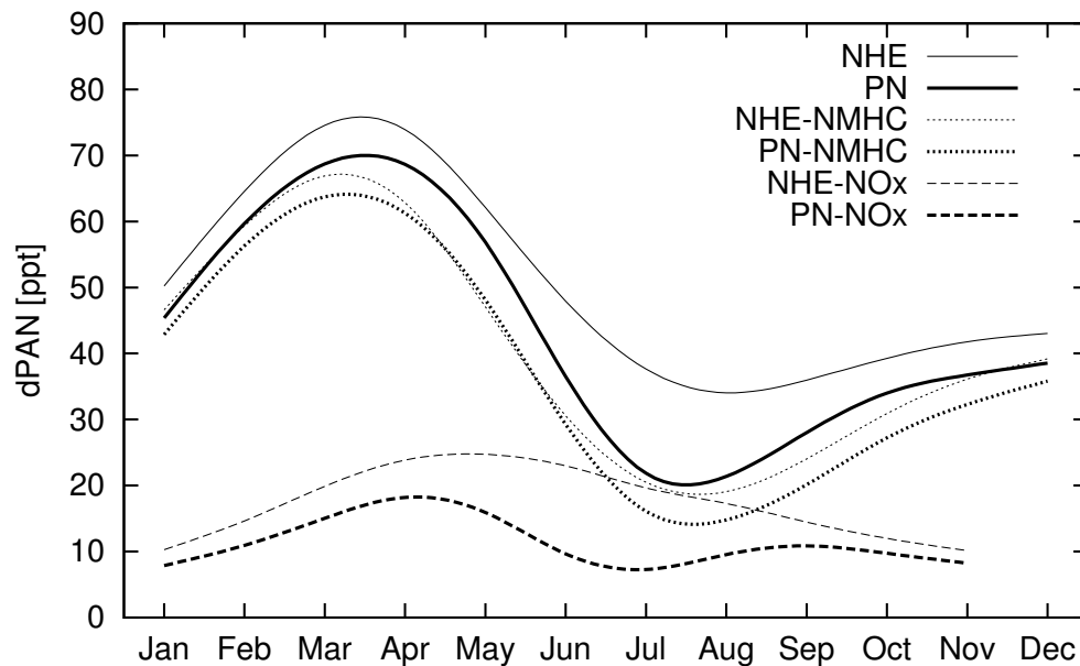
Fig. 7. Individual contributions of road traffic emissions to PAN in two regions: (1) mid-latitudes near the surface (NHE; 30° N–60° N, below 750 hPa) and (2) arctic regions (PN; 68° N–90° N, below 550 hPa); total (solid), NMHCs (dotted), NO x (dashed).
