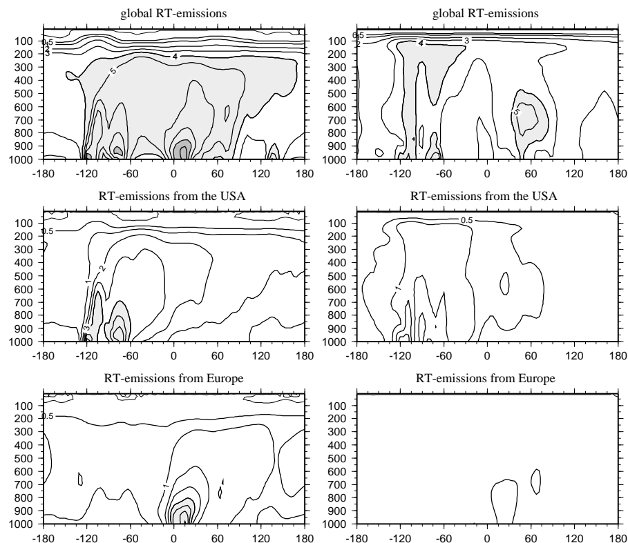
Fig. 9. Contributions [%] of road traffic (RT) emissions to meridionally averaged ozone: global emissions (upper), emissions from the USA (middle) and emissions from Europe (lower) in July. Mid-latitudes denote meridionally averaging over 30° N–60° N and northern tropics over Equator–30° N; isolines distance 1%, plus one additional at .5%.
