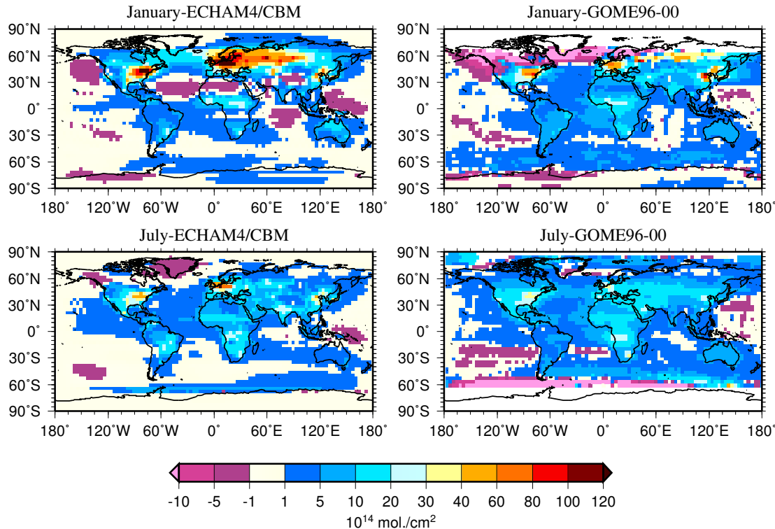
Fig. 2. Tropospheric NO 2 columns [ 10^{14} mol. cm -2 ] derived from GOME satellite data (right) (Richter and Burrows, 2002) and ECHAM4/CBM model simulations (left) for January (top) and July (bottom).
