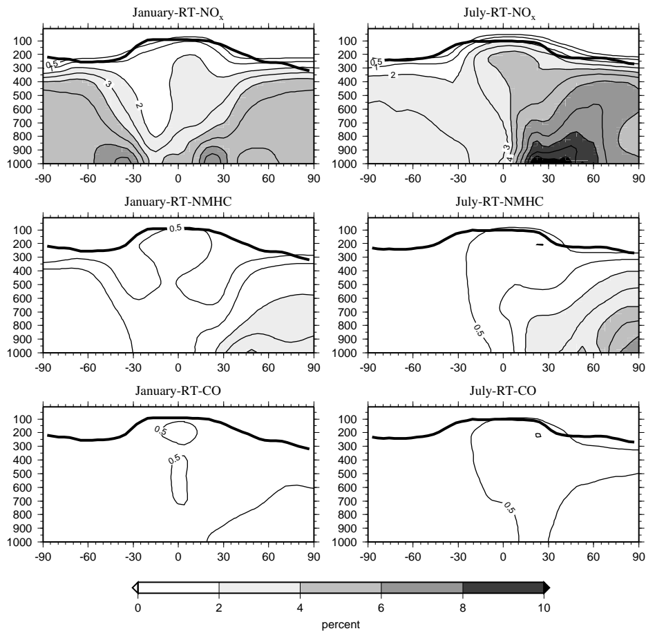
Fig. 6. Contributions [%] of individual road traffic emissions – \text{NO}_x (upper), NMHCs (middle) and CO (lower) to atmospheric distribution of ozone. Isolines are equidistant with 1% difference, plus one additional line for 0.5%.
