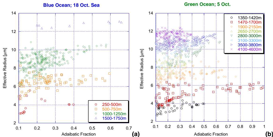
Fig. 12. The dependence of r_e on the adiabatic fraction for all measurements done in the same flight leg, grouped by the different heights (above sea level). Panels (a), (b), (c) and (d) display the measurements of representative flight legs for the Blue ocean, Green ocean, Transition and Polluted regimes, respectively. Each point represents one measurement averaged on circa 40 m of horizontal flight. It can be seen that within each group of heights, r_e is quite robust and also that its value is generally increasing with increasing height, for all regimes.
