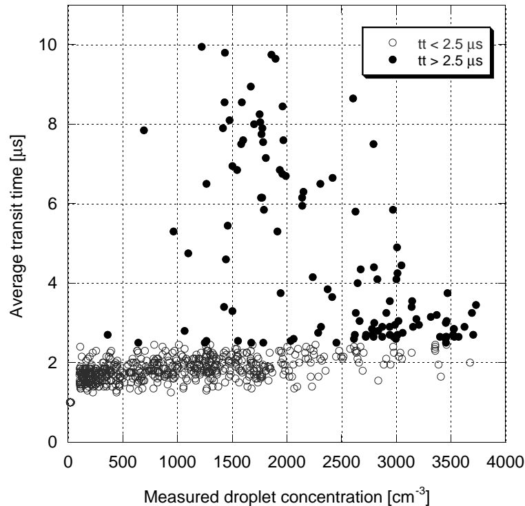
Fig. 4. The average droplet transit time ( tt ) across the laser beam in the FSSP-100 instrument versus the droplet concentration measured by the FSSP while flying in heavily polluted clouds around 19:00 UTC on 4 October 2002. Each point represents the average value along half-a-second of flight ( \sim 40 m). Measurements with tt larger than 2.5 \mu\text{s} are suspected to be significantly affected by the “coincidence problem” and are marked with bold points, whereas measurements with a smaller tt are marked with circles.
