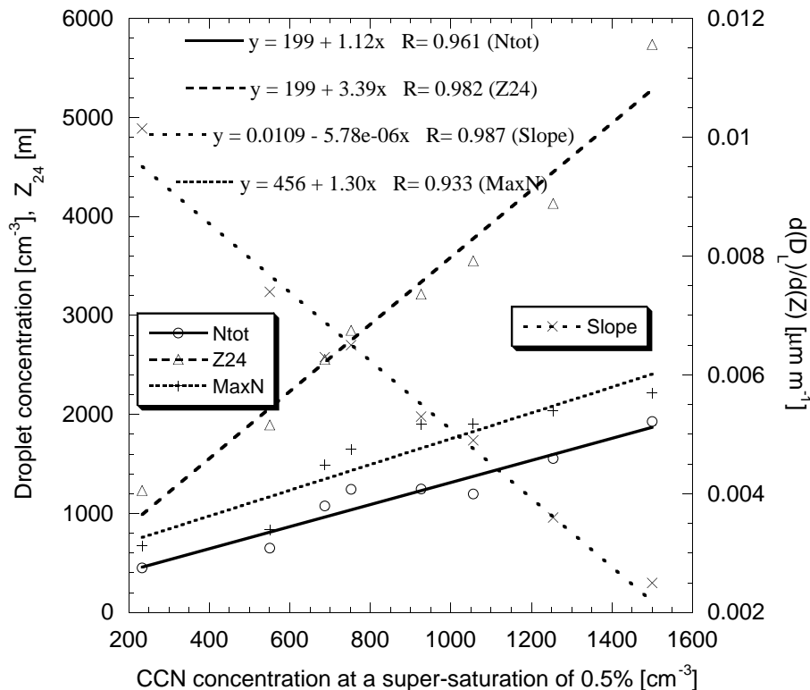
Fig. 9. The relations between CCN concentration at 0.5% SS and four FSSP derived micro-physical parameters: Ntot – the average droplet concentration, Z_{24} – the required cloud depth for the onset of warm rain, MaxN – averaged maximum droplet concentration and Slope – the derivative of D_L with height. Each point represents one complete profile, which is based on at least five cloud penetrations at a range of heights of more than 1 km. Clear linear relations between these independent measurements are seen for all variables.
