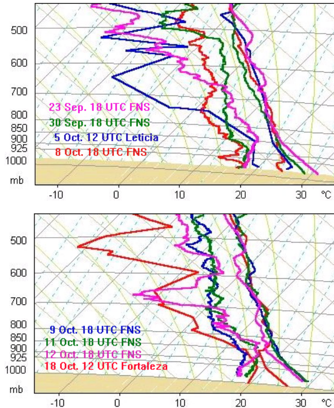
Fig. 3. Temperature ( T ) and dry temperature ( T_d ) profiles ( T_d is to the right of T for each profile represented by a different color) on a Tephigram as derived from radiosonde measurements from all dates and near all places where below-cloud CCN measurements were done. Notice the small variance in T above 850 hPa height.
