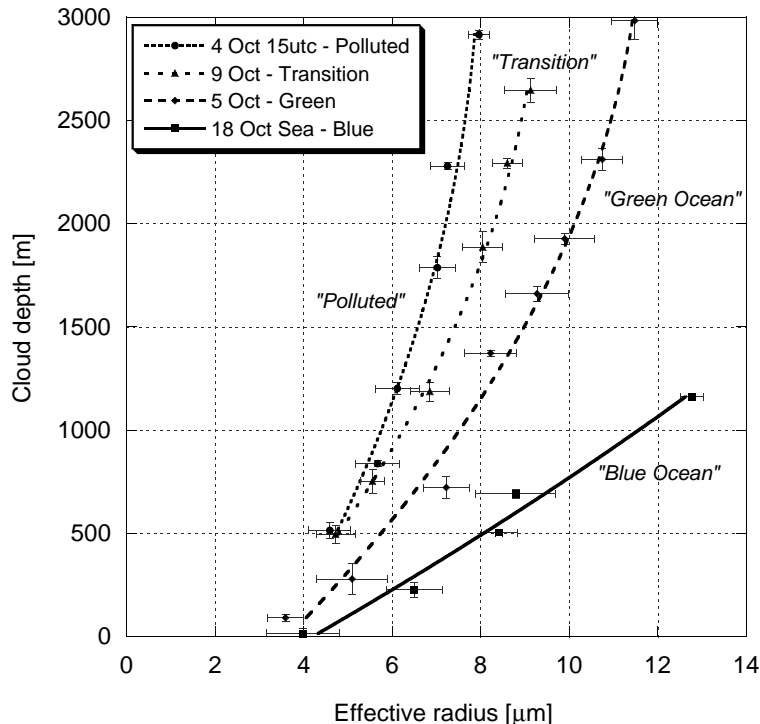
Fig. 13. The growth of r_e with cloud depth for different flight legs from the different regimes. Each point shows the average r_e and the average cloud depth based on the altitude-grouping and the data shown in Fig. 12 for “all” adiabatic fractions. The standard deviations for both r_e and the cloud depth are shown as well, in order to see whether there are significant differences between the different regimes’ r_e profiles and whether their standard deviations overlap. The standard deviations for the cloud depth are quite small because of the horizontal cloud-penetrations at discrete heights. It can be seen that all four profiles start with r_e of \sim 4 \mu\text{m} , but then there is a divergence further up in the cloud, so that at cloud depths of 1500 m and above there is no overlap in the standard deviations of r_e , despite not using all adiabatic fractions.
