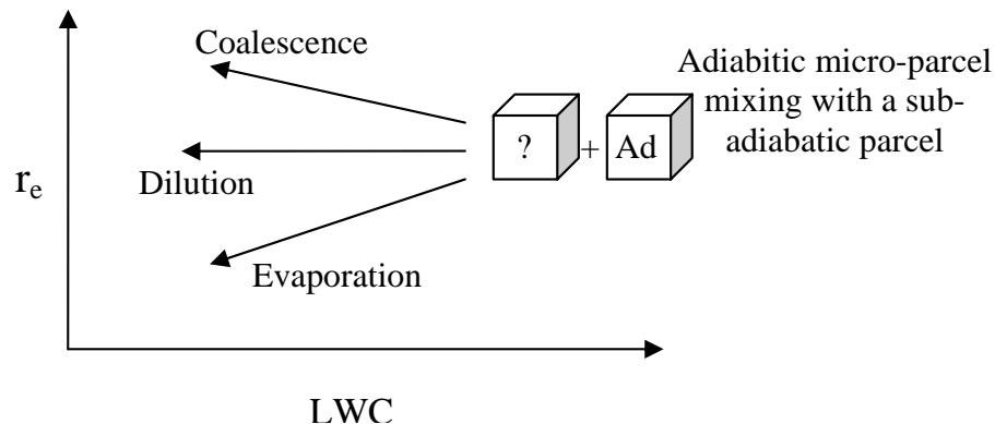
Fig. 14. Schematic illustration of the probable effects of the evaporation, dilution and coalescence processes on the r_e -LWC relation when an adiabatic parcel mixes with another sub-adiabatic parcel. The box marked with “Ad” represents the adiabatic parcel and its location on the r_e -LWC plane is meaningful, while the box marked with a question mark represents the sub-adiabatic parcel and its location on the plane is variable although its LWC has to be smaller than the adiabatic parcel (when there are no falling-from-above precipitation particles). The final location of the newly mixed parcel on the r_e -LWC plane will be determined by the relative importance of the above mentioned processes.
