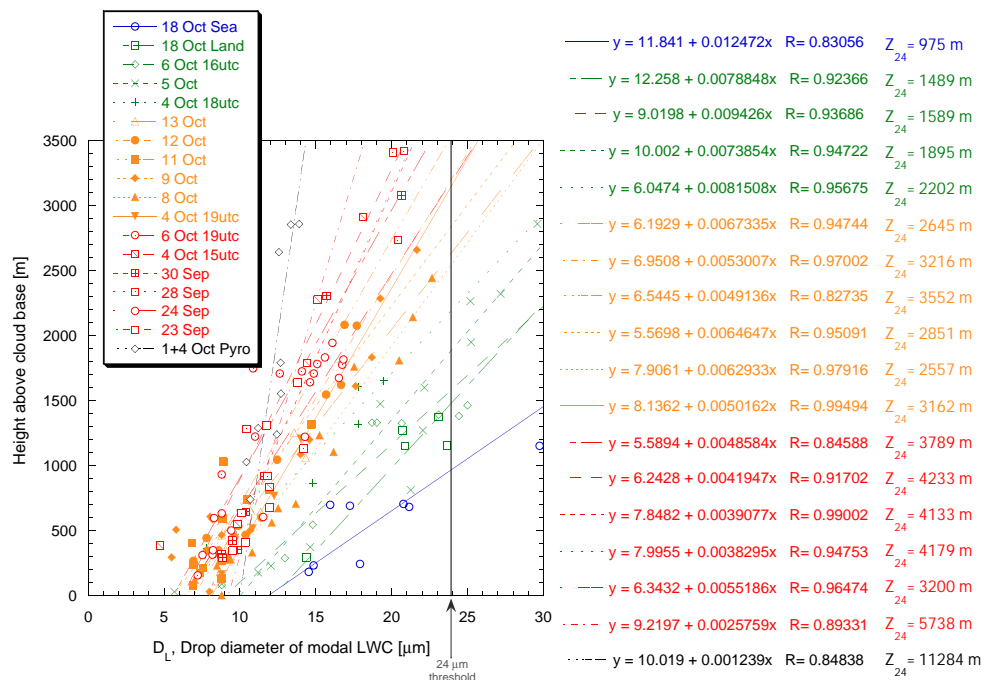
Fig. 8. The growth of D_L with cloud depth for all flights that included a vertical cloud profile of at least 1 km depth. Each point represents the averaged D_L for one horizontal penetration at a certain height. The color scheme is based on the pollution regime in the following way: in blue are Blue ocean measurements, in green – Green ocean, in orange – Transition regime, in red – Polluted regime and in black – Pyroclouds. Each profile was named after its date and if necessary, its time and additional self-explanatory information. The order of the profiles' appearance in the legend corresponds to the order of the equations of the best-fit linear regressions shown to the right. The 24 \mu\text{m} threshold for the onset of warm rain is marked on the figure. The cloud depth at which D_L crosses this threshold for each profile – Z_{24} , is shown at the extreme right. It can be seen that in the more polluted regimes, the clouds need to have a larger vertical extent in order for D_L to reach the 24 \mu\text{m} warm rain threshold, compared to the clouds in the cleaner regimes.
