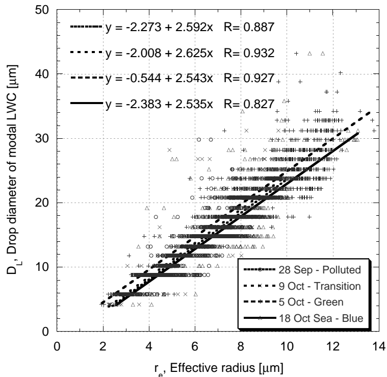
Fig. 7. The relation between the drop diameter of modal LWC ( D_L ) and the effective radius ( r_e ) for four representative flight legs in the different pollution regimes. Each point represents half-a-second measurement. It can be seen that there is quite a strong relation between these variables and that this relation is not strongly dependent on the pollution regime. The discrete nature of the D_L values, due to the use of size-bins by the FSSP, is also noticeable.
