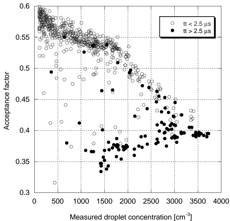
Fig. 5. The acceptance factor ( af – see text for definition) as reported for each measurement versus the FSSP droplet concentration for the exact same measurements as presented in Fig. 4. Measurements with tt larger than 2.5 \mu\text{s} (see Fig. 4) are marked with bold points and show significantly smaller af than those with smaller tt (in circles).
