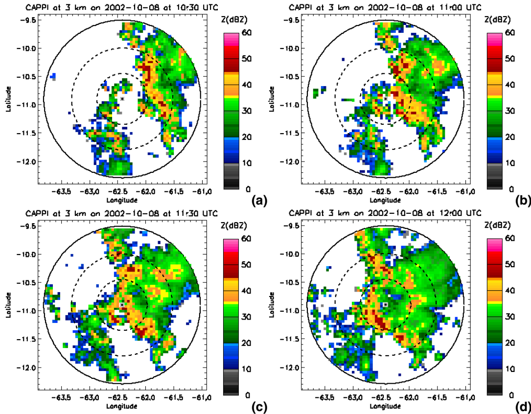
Fig. 2. A sequence of precipitation radar reflectivity images at a constant height of 3 km around FNS (located at the asterisk in the center of each panel) for 30 min increments, starting at 10:30 UTC 8 October 2002 (panels (a) through (d)). It can be seen that a squall line, seen as the high reflectivity areas (yellow and red) located to the east of FNS at 10:30 UTC, is moving westwards and crosses FNS at around 1130 UTC (panel (c)). The passing of the squall line is linked to the drastic drop in \text{PM}_{2.5} concentration at the same time shown in Fig. 1.
