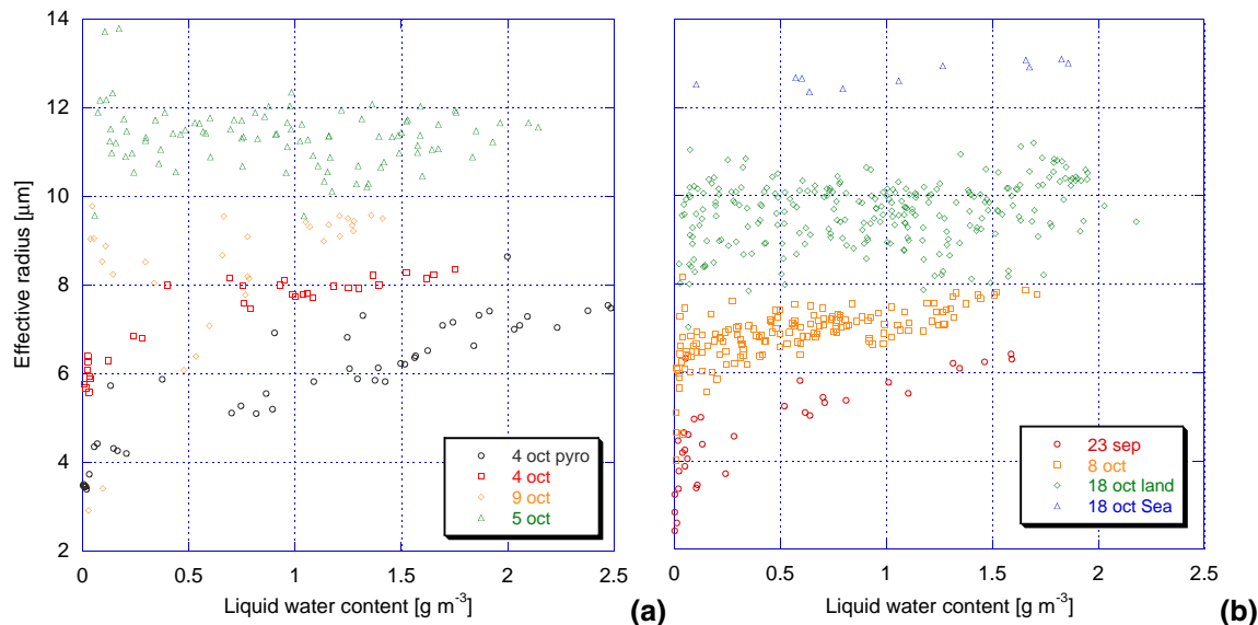
Fig. 11. The dependence of the effective radius ( r_e ) on the Liquid Water Content (LWC) for the different pollution regimes (each represented by one flight leg) at a nearly constant cloud depth of 2700 m in panel (a) and of 1200 m in panel (b). Each point represents one measurement averaged on circa 40 m of horizontal flight. The color scheme is the same as in Fig. 8. r_e shows only a small variance compared to LWC and its value is higher for the cleaner regimes when looking at a nearly constant height.
