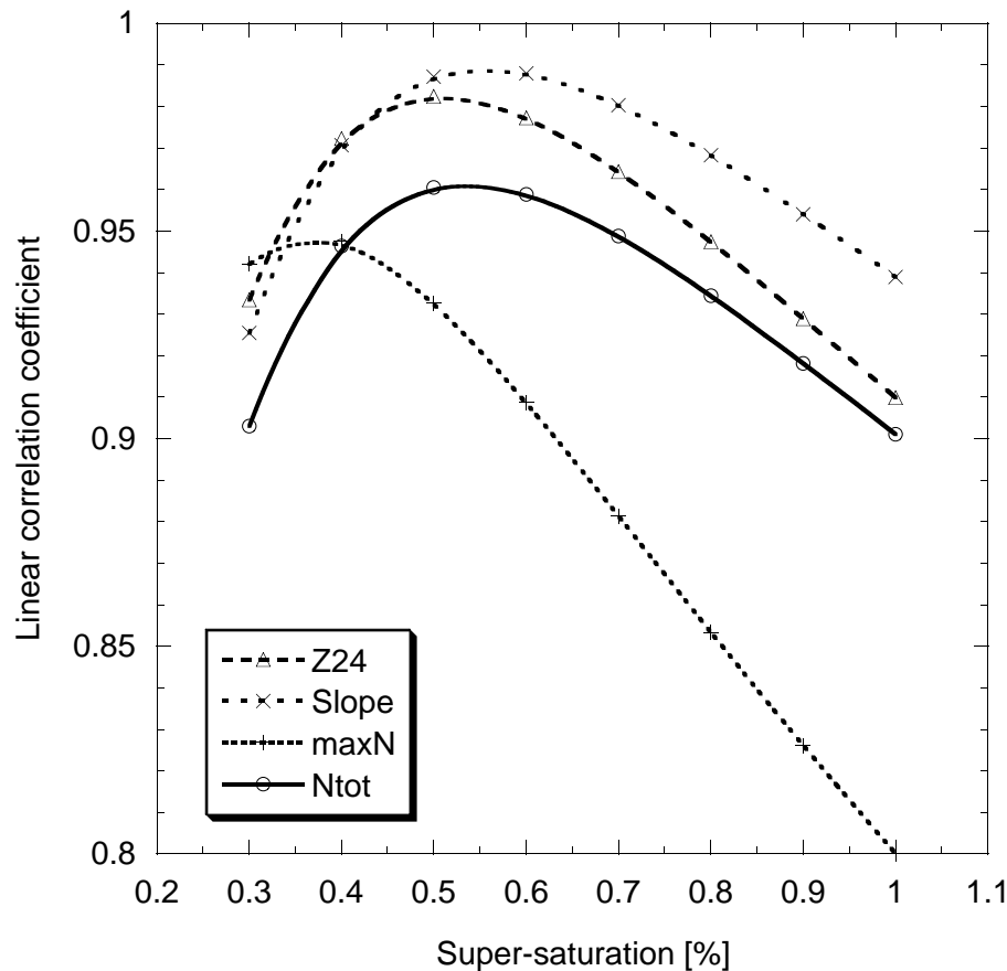
Fig. 10. The linear correlation coefficients between each microphysical parameter shown in Fig. 9 and the interpolated CCN concentration at different super-saturations (SS) that was based on the measurements of the CCNC. It can be seen that the correlation coefficients peak at SS of 0.5–0.6% for all variables but MaxN .
