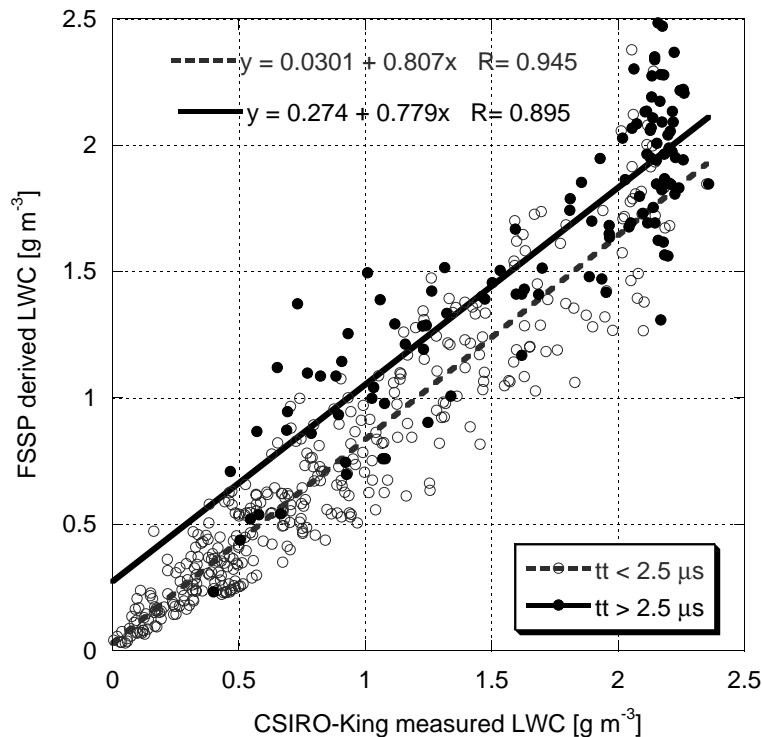
Fig. 6. The relation between FSSP-derived (cloud) Liquid Water Content (LWC) and the LWC measured by the hot-wire King probe for the same measurements as presented in Figs. 4 and 5. Again, the bold points represent the measurements with a tt larger than 2.5 \mu\text{s} . A linear regression line is shown for each group of measurements (according to their tt ) suggesting similar slopes (p-value is 0.94 when testing for equal values) but the intercepts are slightly different (p-value is 0.024).
