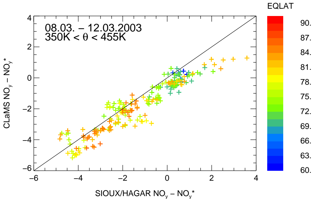
Fig. 8. Comparison of \text{NO}_y\text{-NO}_y^* simulated by CLaMS and derived from SIOUX and HAGAR observations on Geophysica on 8 and 12 March 2003 for equivalent latitudes above 60^\circ\text{N} . The color of the symbols denotes the equivalent latitude of the observation location.
