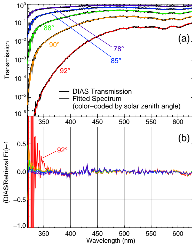
Fig. 3. Goodness of fits. (a) DIAS transmission spectra at five SZAs, 78^\circ – 92^\circ , from 6 February 2003 DC-8 flight, with fitted spectra overlaid. (b) Relative transmission difference, (\text{DIAS}/\text{fitted spectra}) - 1 , with the same SZA color-coding as (a).
