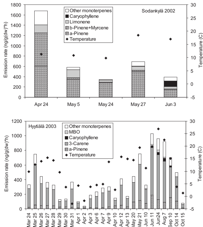
Fig. 1. Average noontime emission rates measured in April–June 2002 in Sodankylä and in March–October 2003 in Hyytiälä. Other monoterpenes comprises camphene, sabinene, 1,8-cineole, linalool, and bornyl acetate in Sodankylä, and camphene, sabinene, \beta -pinene+myrcene, terpinolene, limonene, 1,8-cineole, \beta -phellandrene, terpinolene, and bornyl acetate in Hyytiälä. The average temperature during the measurements (solid diamonds) is shown on the right hand axis. Note that the x-axis is not in scale because the averages for each measurement day are shown at regular intervals.
