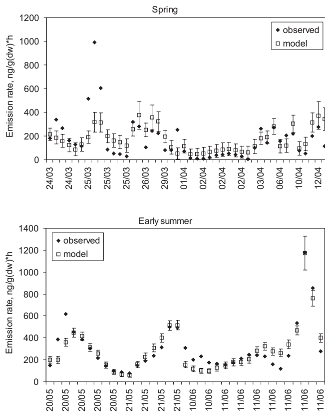
Fig. 3. (a) Measured and modelled \Delta^3 -carene emissions in Hyytiälä in spring and early summer in 2003. Note that the x-axis is not in scale because each measurement is shown using regular intervals. The error bars indicate the 95% confidence limits of the nonlinear regression fit.
