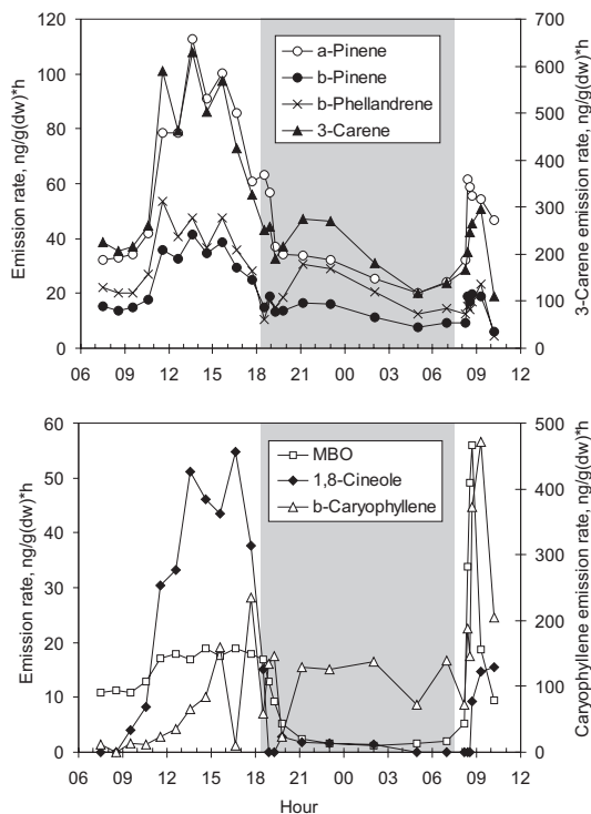
Fig. 2. Variation of the VOC emission rates of Scots pine in Hyttiälä during the darkening experiment 7–8 on August 2003. The branch was covered from light at 6:30 p.m. on the 7th and the cover was removed at 7:00 a.m. on the 8th.
