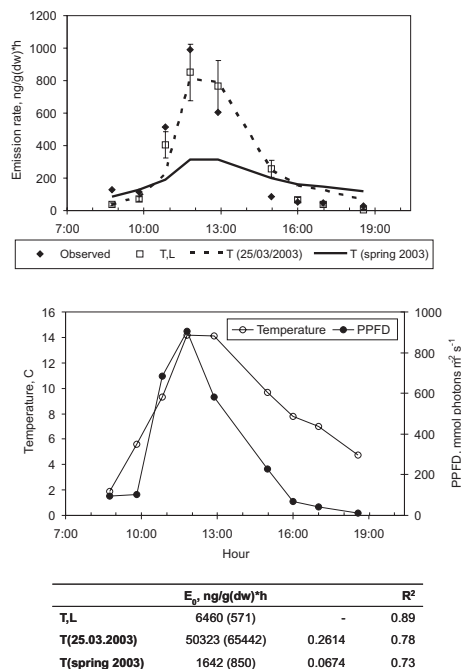
Fig. 4. Measured and modelled \Delta^3 -carene emissions in Hyytiälä on 25 March 2003 (upper panel). The light and temperature dependent algorithm (Eq. 4) is denoted by T, L. The temperature algorithm (Eq. 3) is denoted by T. T (25/03/2003) is fitted to the data of 25 March only, while T (spring 2003) refers to the seasonally fitted algorithm (same as in the upper panel of Fig. 3a). The error bars indicate the 95% confidence limits of the nonlinear regression fit to T,L. The lower panel shows the temperature and the photosynthetically active radiation (PPFD). The standard emission potentials (30°C) obtained with the different models and the corresponding parameters are given under the figure.
