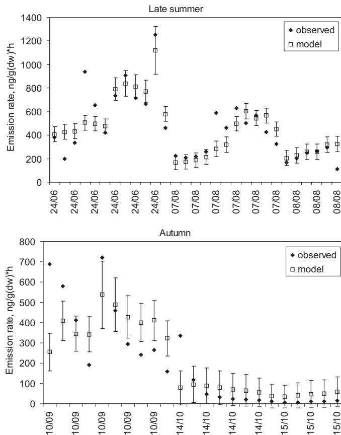
Fig. 3. (b) Same as Fig. 3a but for late summer and autumn in 2003.
