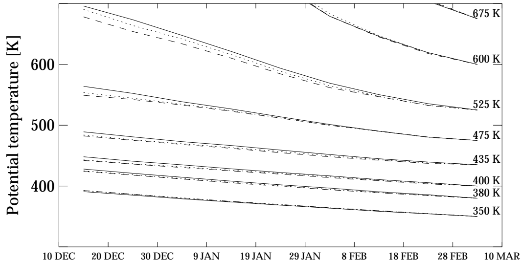
Fig. 3. Diabatic cooling during the winter 2002/2003 calculated along Lagrangian trajectories ten days back in time for air masses ending in the vortex. Solid line: vortex collar. Dotted line: vortex middle. Dashed line: vortex centre.
