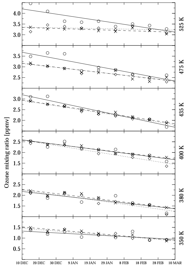
Fig. 5. Ozone mixing ratios, averaged over ten-day intervals and over vortex areas (collar, middle and centre), corrected for diabatic descent and transport into the vortex. Linear best fits to the data are shown for each area and each of six \theta levels. Circles: vortex collar. Diamonds: vortex middle. Crosses: vortex centre. Solid lines: vortex collar. Dotted lines: vortex middle. Dashed lines: vortex centre.
