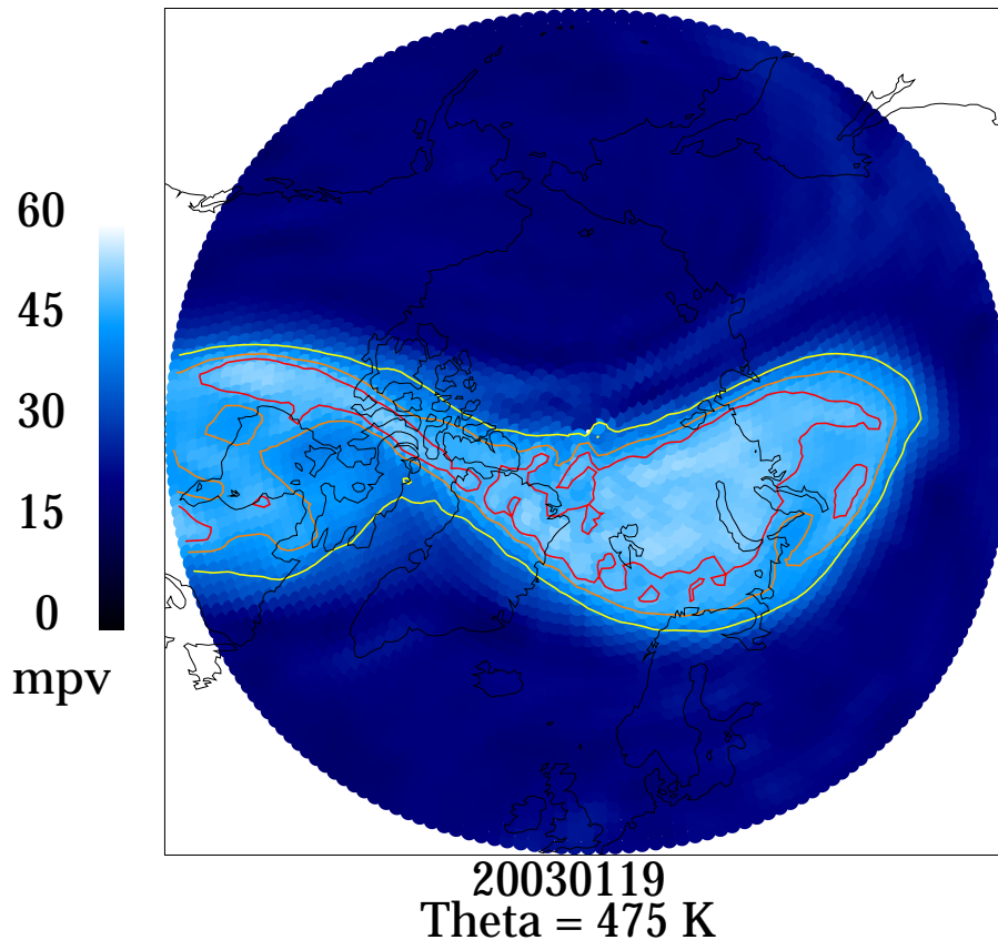
Fig. 1. Modified potential vorticity MPV north of 50°N in units of PVU at \theta=475 K on 19 January 2003 from ECMWF analyses. The yellow contour line shows the vortex edge, the orange contour line shows the limit between the vortex collar and middle and the red contour line shows the limit between the vortex middle and centre.
