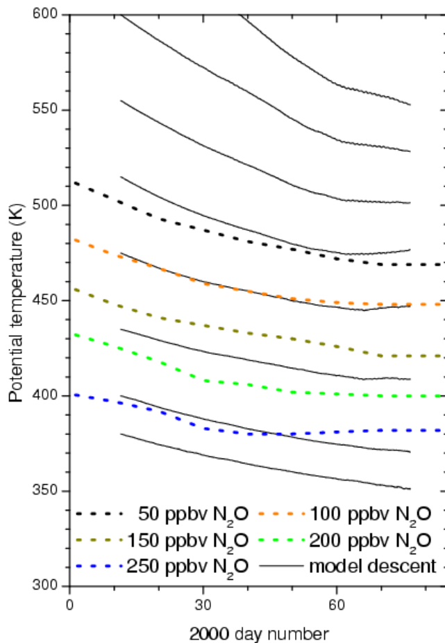
Fig. 2. Comparison of the N 2 O descent lines from Greenblatt et al. (2002) and our modelled diabatic descent based on climatological ozone for the winter 1999/2000 vortex.
