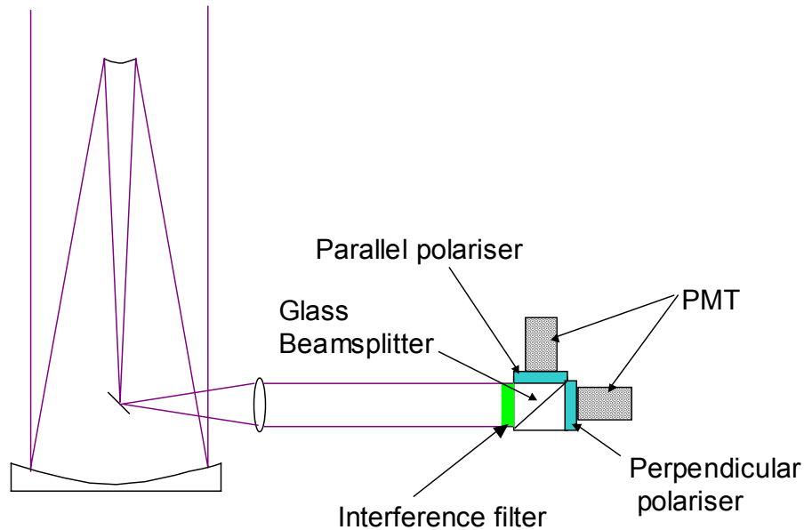
Fig. 1. Schematic of lidar receiver.
