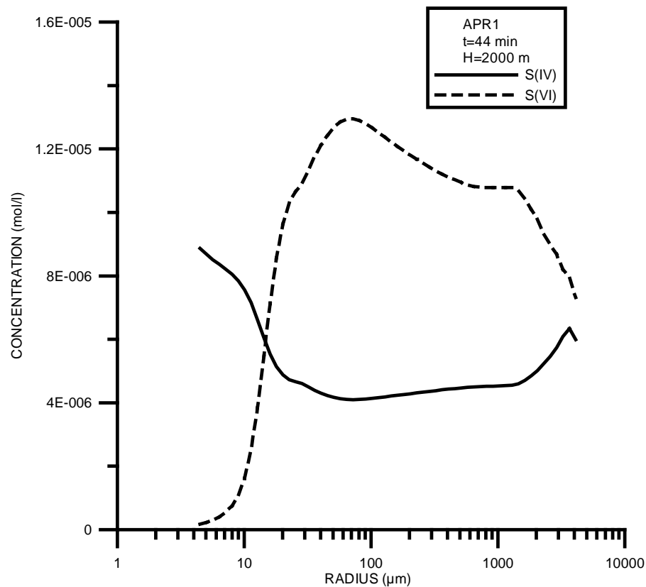
Fig. 8. S(IV) and S(VI) aqueous phase concentrations at 2000 m for the case with aqueous-phase oxidation, an initial formic acid gas-phase concentration of 1ppb and high (20 ppb) SO 2 ambient concentration (APR1), after 44 min of simulation.
