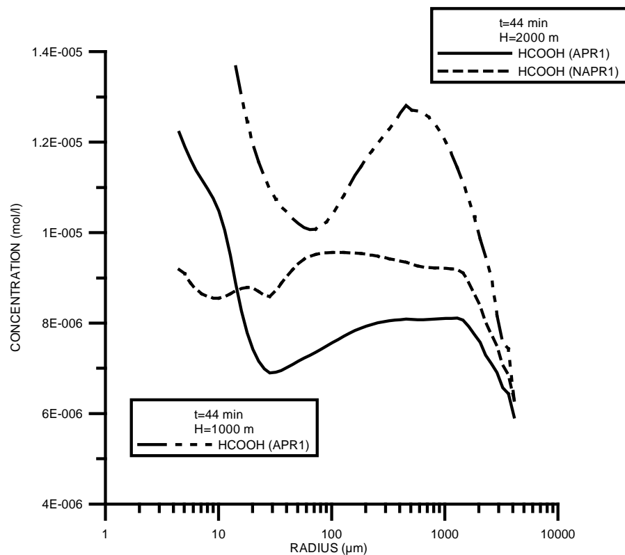
Fig. 9. HCOOH aqueous phase concentration at two different inclusion levels (1000 and 2000 m), for the cases with aqueous phase oxidation, and no aqueous phase oxidation, an initial formic acid gas-phase concentration of 1 ppb and high (20 ppb) SO 2 ambient concentration (APR1, NAPR1), after 44 min of simulation.
