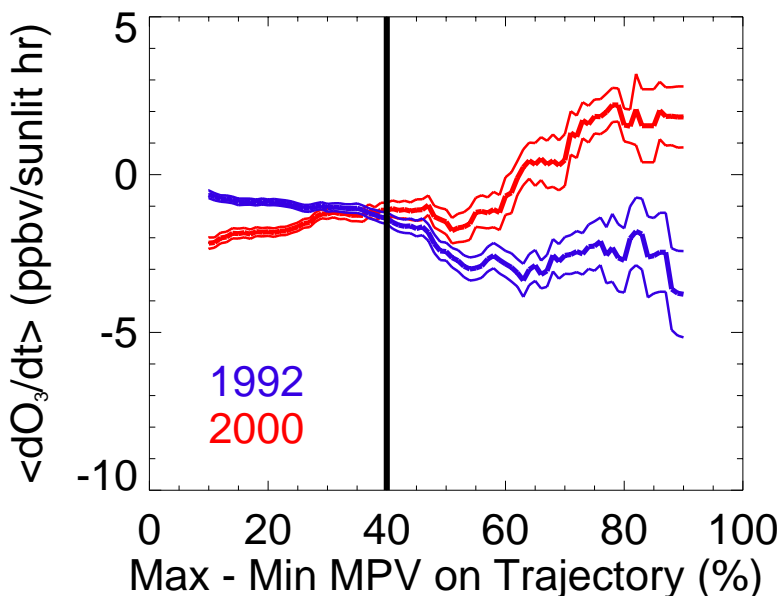
Fig. 3. The sensitivity of the ozone loss rate on the maximum minus minimum PV difference along the back trajectory (see text) is explored for AASE-2/EASOE (blue) and SOLVE/THESEO 2000 (red). The thick lines represent the mean values while the thin lines represent the means plus and minus one standard deviation.
