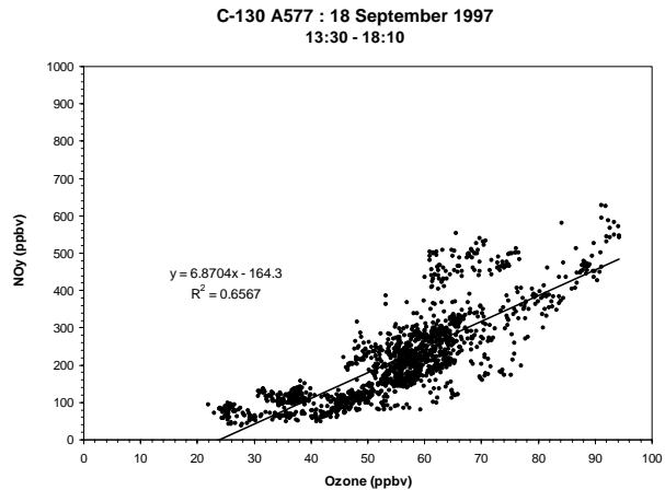
Fig. 11. Correlation plot for NO y against ozone for flights A534 (in spring, upper panel) and A577 (in summer, lower panel). Note the difference in the slopes between spring and summer for plots with similar correlation coefficients.
