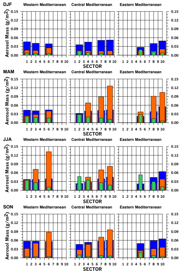
Fig. 12. Mean seasonal ( S =DJF, MAM, JJA and SON) maritime, continental and desert dust mass loads ( \text{g}/\text{m}^2 ; blue, green and orange histograms, respectively) in the ten sectors (SEC) of Fig. 10, shown separately for Western (SEC=1, 3, 6), Central (SEC=2, 4, 7, 9) and Eastern (SEC=5, 8, 10) Mediterranean (left, central and right column, respectively).
