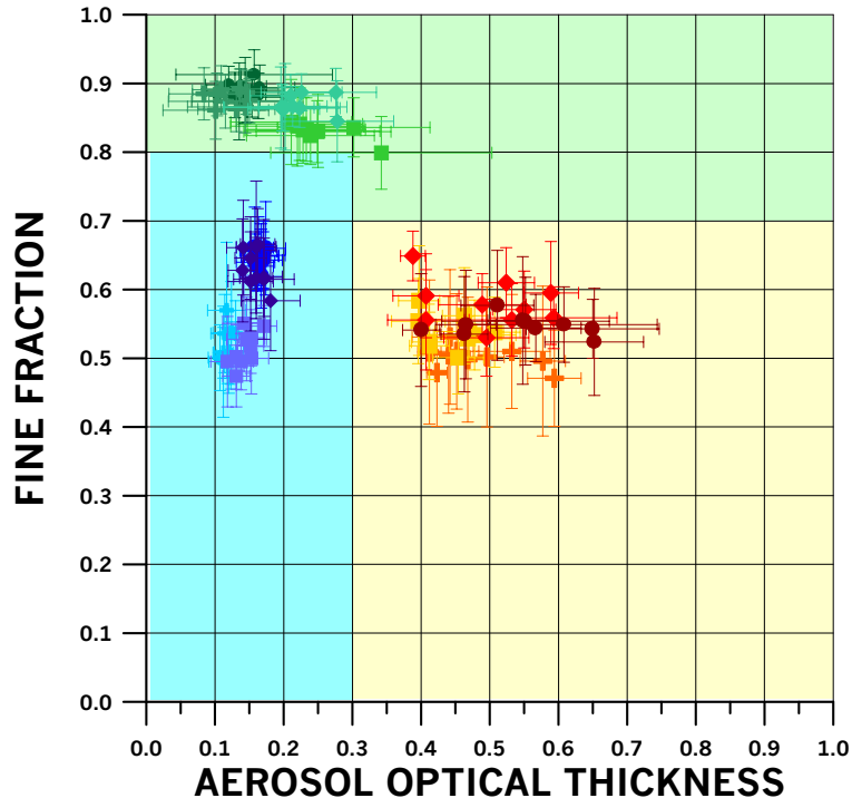
Fig. 11. Mean seasonal FF vs. AOT values characterizing each aerosol type in the ten Mediterranean sectors of Fig. 10 (i.e. FF_{S,type \text{ in } SEC} vs. AOT_{S,type \text{ in } SEC} data). Blue, green and red points refer to maritime, continental and desert dust aerosol, respectively. Different symbols are used to indicate the different seasons (i.e. crosses, bullets, diamonds and squares refer to DJF, MAM, JJA and SON, respectively). The aerosol mask thresholds of Fig. 1 are also indicated in the graph.
