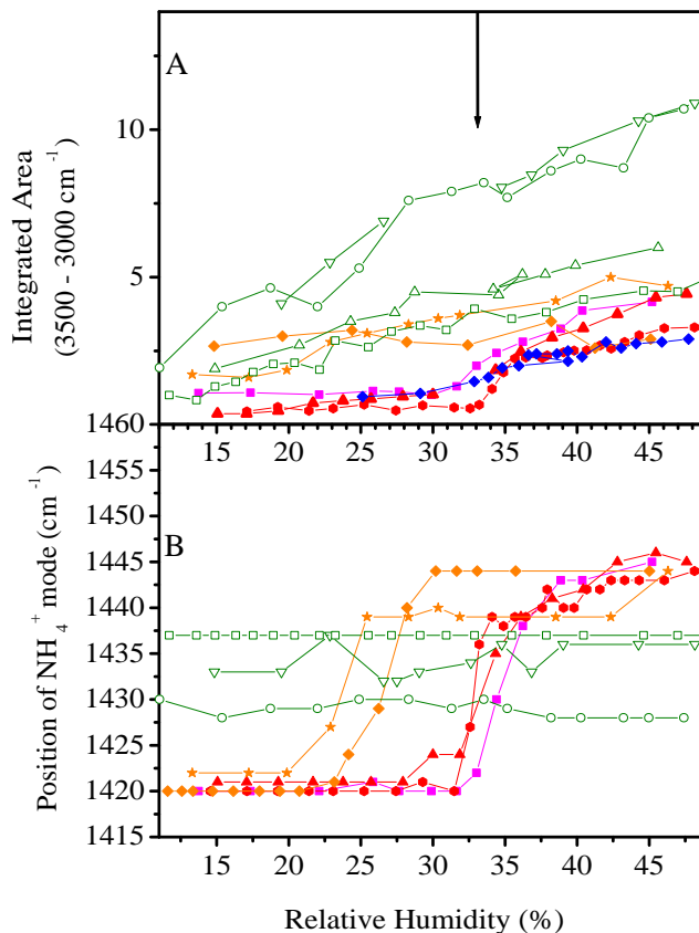
Fig. 4. Efflorescence mode experiments. A: Integrated area ( 3500\text{--}3000\text{cm}^{-1} ) due to condensed phase water as a function of RH. B: Position of ammonium mode ( \text{NH}_4^+ ). Composition key: f_{MA} (symbol): 0.00 (pink \blacksquare ); 0.01 (red filled hexagon); 0.06 (red filled \Delta ); 0.10 (orange filled \diamond ); 0.25 (orange filled * ); 0.40 (green \nabla ); 0.49 (green \square ); 0.60 (green \circ ); 0.75 (green \Delta ); 0.92 (blue filled \diamond ); Arrow: \downarrow:ERH_{AS} .
