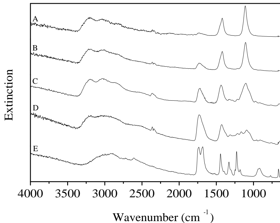
Fig. 1. Infrared spectra of five compositions of ammonium sulfate (AS) – malonic acid (MA) solutions at <1% RH. Compositions as dry fraction of MA ( f_{MA} ): A: 0.10; B: 0.25; C: 0.49; D: 0.75; E: 0.90.
