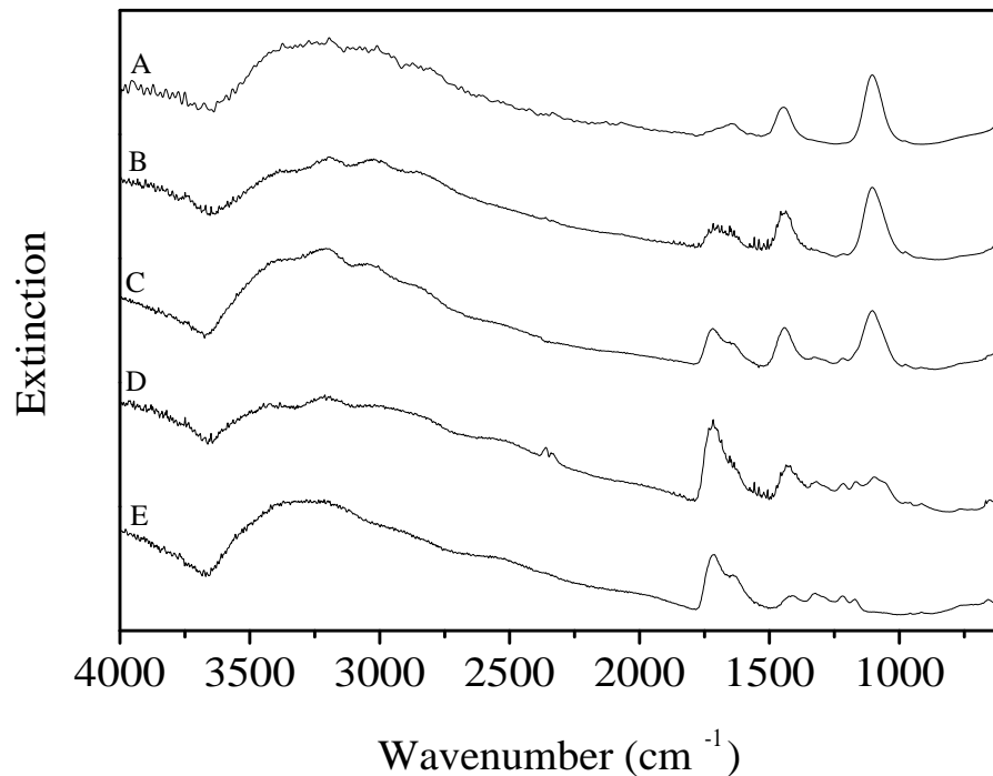
Fig. 2. Infrared spectra of five compositions of ammonium sulfate (AS) – malonic acid (MA) solutions at >80% RH. Compositions as dry fraction of MA ( f_{MA} ): A: 0.10; B: 0.25; C: 0.49; D: 0.75; E: 0.90.
