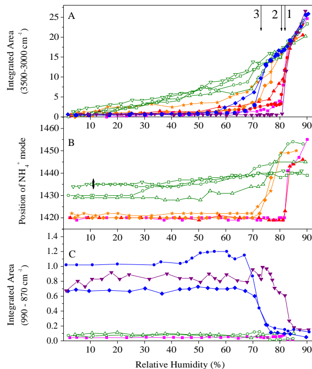
Fig. 3. Deliquescence Mode Experiments. A: Integrated Area (3500–3000 cm -1 ) due to condensed phase water as a function of RH. B: Position of ammonium mode (NH 4 + ). C: Integrated area of malonic acid mode between 990–870 cm -1 . Composition key: f_{MA} (symbol): 0.00 (pink ■); 0.01 (red filled hexagon); 0.06 (red filled Δ); 0.10 (orange filled ◇); 0.25 (orange filled *); 0.40 (green ▽); 0.49 (green □); 0.60 (green ○); 0.75 (green Δ); 0.92 (blue filled ◇); 0.98 (blue filled ○); 1.00 (purple filled ▽). Arrows: 1:DRH AS ; 2:DRH MA ; 3:EDRH; ↑: Uncertainty in peak position resolution.
