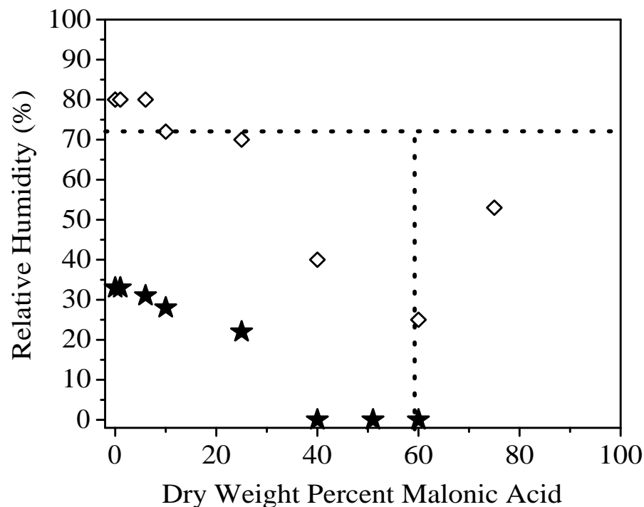
Fig. 5. Phase transition points of ammonium sulfate in ammonium sulfate-malonic acid mixtures as determined by shift in \text{NH}_4^+ mode: Ammonium sulfate observed to go into solution, 283 K ( \diamond ); Crystallization of ammonium sulfate, 293 K (black filled \star ). Eutonic composition and EDRH for ammonium sulfate – malonic acid – \text{H}_2\text{O} ternary system at 283 K is shown with the dashed line (Brooks et al., 2002). See text for details.
