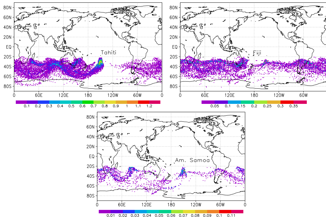
Fig. 6. Trajectory density (see its definition in the text) of trajectories arriving at Tahiti, Fiji and Am. Samoa at altitudes of 800 to 500 hPa in September 1999 while being in the stratosphere. It can clearly be seen that air masses arriving at Tahiti are more subject to stratospheric influence than trajectories arriving at Fiji or Am. Samoa.
