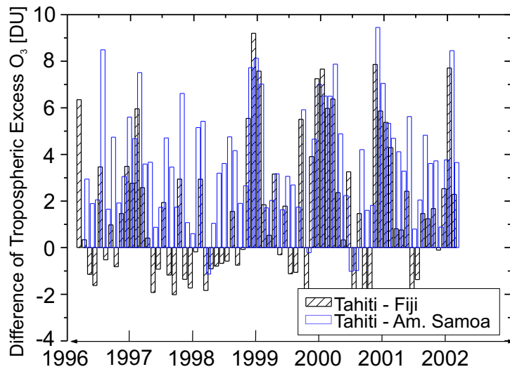
Fig. 1. Calculated differences of monthly mean values for tropospheric excess column amounts between Tahiti and Am. Samoa as well as between Tahiti and Fiji for 1996–2002.
