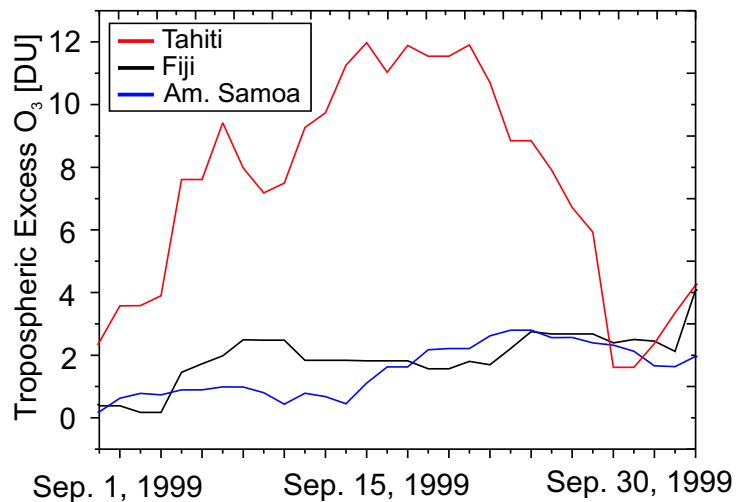
Fig. 2. Time series of the tropospheric excess column of ozone between 1 September to 30 September 1999 for the locations Am. Samoa, Fiji and Tahiti.
