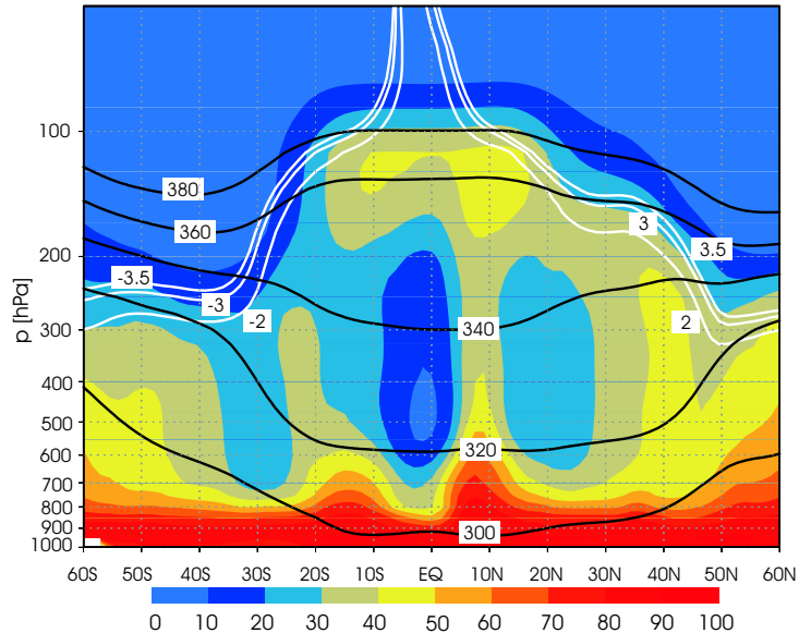
Fig. 5. Zonal average for the Pacific region from 160 to 220° E of relative humidity (color scale, given in percent), potential temperature (black lines, given in K) and potential vorticity (white lines, given in PVU) of September 1999. The relative humidity is denoted by the colorscale, the potential temperature by the black lines and the potential vorticity by the white lines. The latter is shown for absolute values of 2, 3 and 3.5 PVU which represent different tropopause height definitions. The meteorological data is derived from the 40-years reanalysis (ERA-40) of the European Centre for Medium Range Weather Forecasts (ECMWF).
