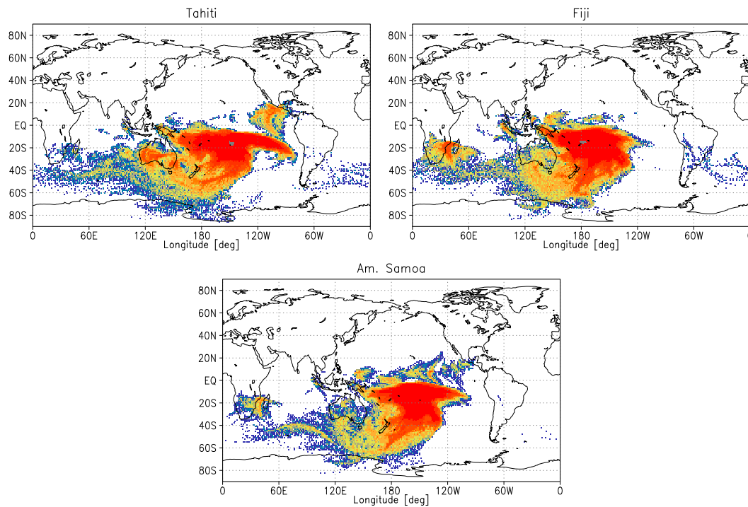
Fig. 3. Density of trajectories arriving above Tahiti, Fiji and Am. Samoa during September 1999 while residing in the planetary boundary layer.
