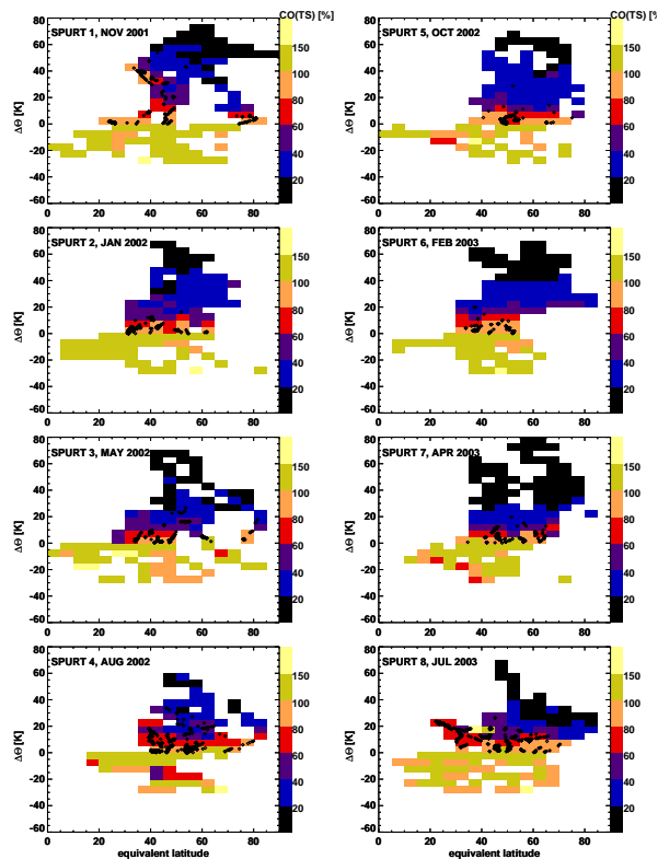
Fig. 6. Tropospheric fraction of CO relative to the respective isentropic tropopause CO-value in Fig. 5 as a function of equivalent latitude and \Delta\Theta above the tropopause (details see text).
