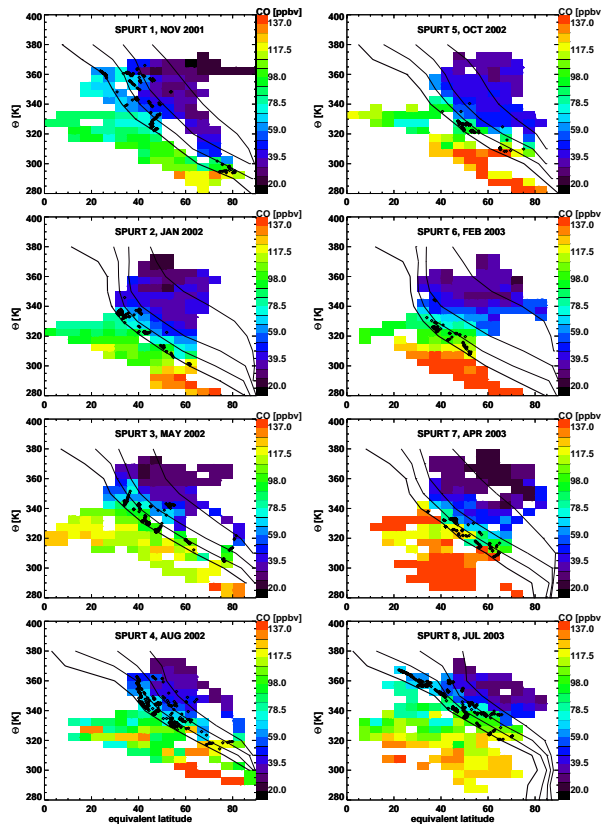
Fig. 5. CO-distribution in equivalent latitude \phi_{eq} - \Theta -coordinates for the whole SPURT-deployment. The thick black line denotes the location of the tropopause PV = 2 PVU-surface, thin lines mark the 4,6 and 8 PVU-contours, respectively. Superimposed are the positions of 10-day backward trajectories indicating TST within ten days before the flights.
