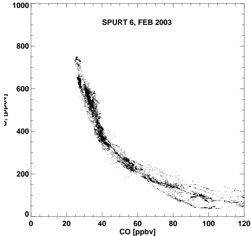
Fig. 3. Scatterplot of CO and ozone for SPURT 6 in February 2003. Taking an ozone threshold of 100 ppbv as an approximation for the tropopause the anticorrelation indicates irreversible cross tropopause mixing. Note, that at O_3 = 300 ppbv the slope abruptly changes indicating a rather sharp transition between different layers.
