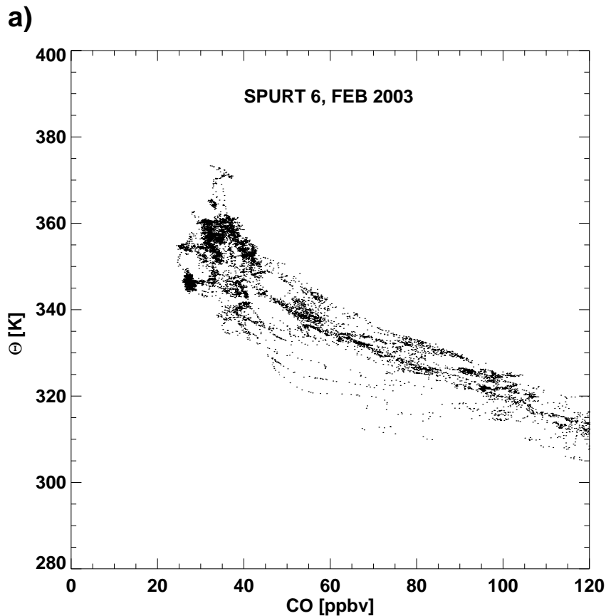
Fig. 4. (a) Complete CO data set obtained during the SPURT 6 missions as a function of (a) potential temperature and (b) potential temperature relative to the local tropopause \Delta\Theta . Note the more compact \Delta\Theta -profile and the rather sharp change of the CO gradient at \Delta\Theta = 25 K. (c) \text{CO}_2 as a function of \Delta\Theta during SPURT 6 showing the same behaviour at \Delta\Theta = 25 K.
