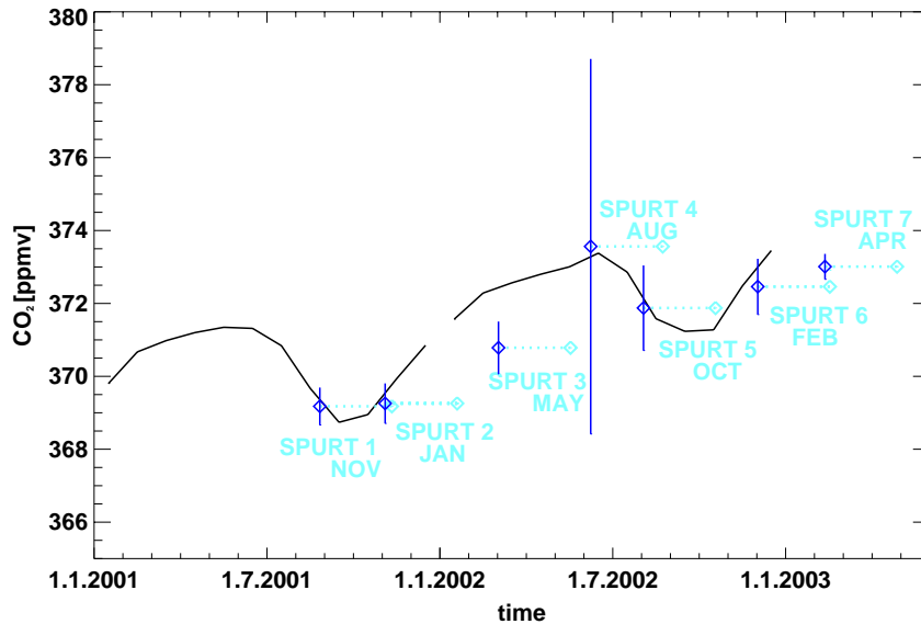
Fig. 8. Tropical CO 2 surface data and tropical tropopause CO 2 -data deduced from SPURT shifted backward in time by 2.5 months (dark blue), light blue: time of measurement. Error bars are deduced from the error of the fit parameters of the N 2 O-CO 2 -correlation for \Delta\Theta > 45 K (details see text).
