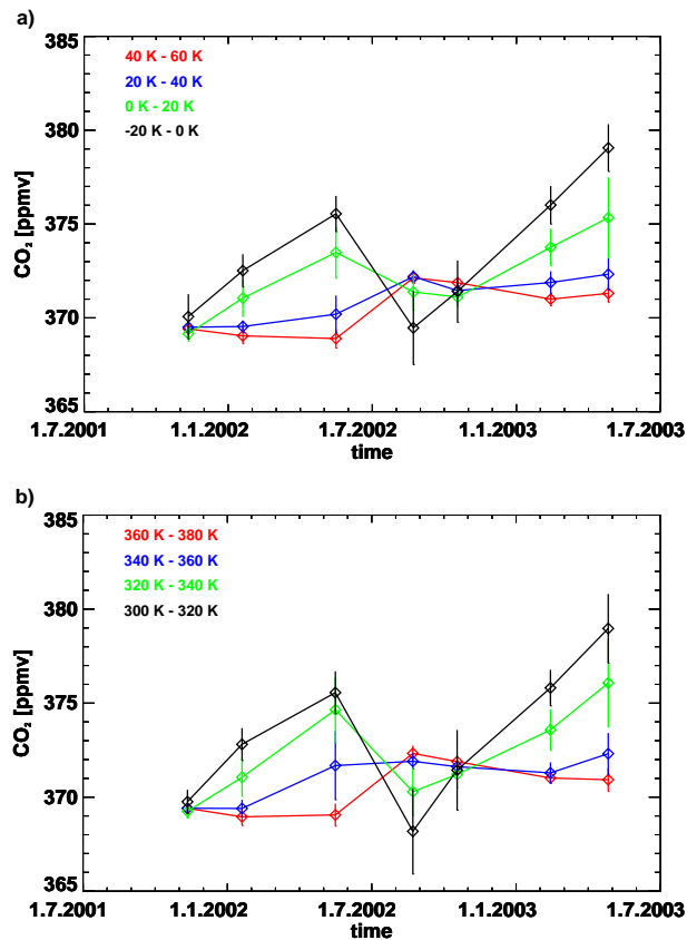
Fig. 7. (a) CO 2 as a function of time and \Delta\Theta above the local tropopause. The phase shift at \Delta\Theta > 20 K is evident. (b) CO 2 on isentropic surfaces. Note the local maximum in summer on the highest isentropic surface of \Theta = 360 K and the negative vertical CO 2 gradient in August 2002.
