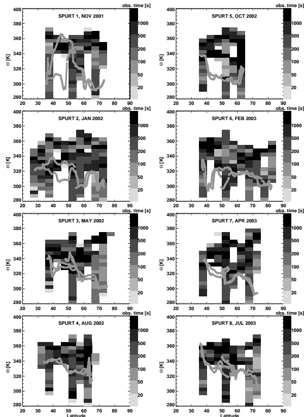
Fig. 2. Data coverage for SPURT as a function of latitude and theta. The location of the local tropopause at the position of the aircraft is superimposed. Note the variability of potential temperature at the tropopause during each deployment.
