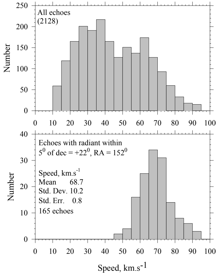
Fig. 10. The distribution of measured speeds for the 2128 echoes observed at the 3 stations and the speed distribution for radiants within 5° of the expected Leonid radiant.
