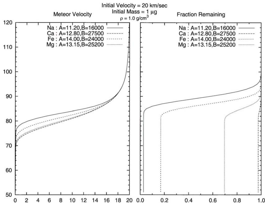
Fig. 1. The ablation of a 1 µg particle entering the atmosphere at 20 km/s.
