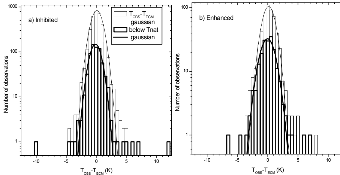
Fig. 1. Histogram of the temperature biases for inhibited (a) and enhanced (b) wave activity. The histograms for temperatures below T_{\text{NAT}} are shown in bold.
