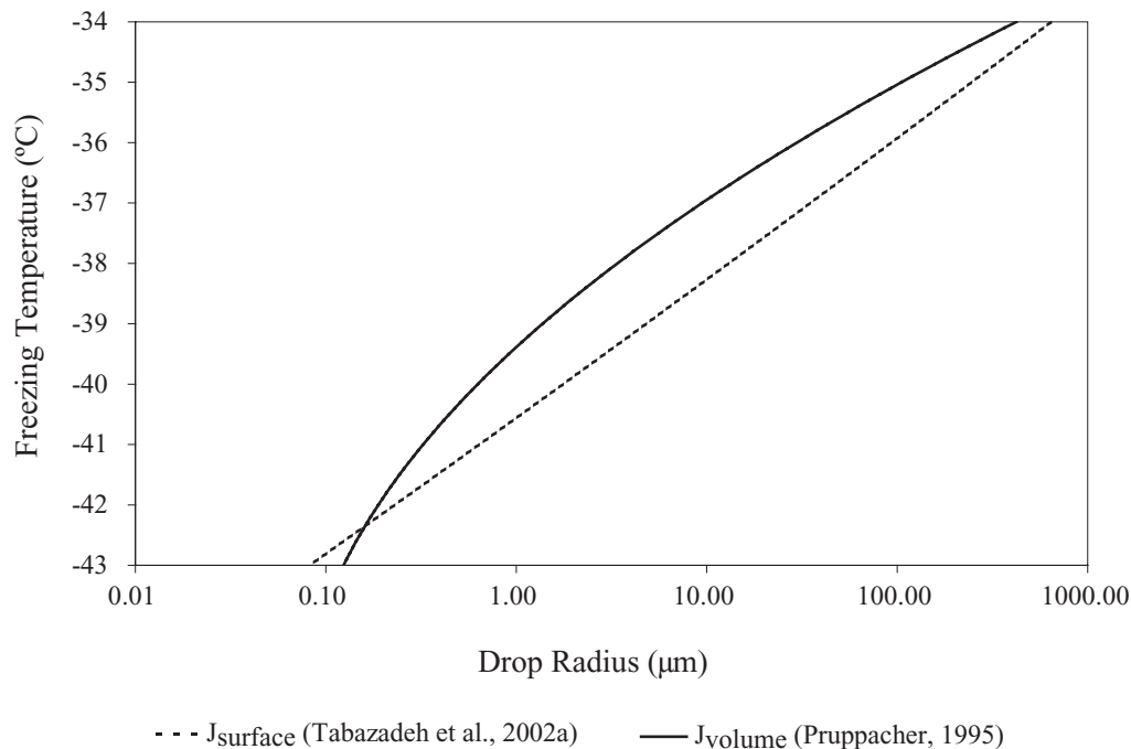
Fig. 1. Estimated freezing temperature ( J=1 \text{ s}^{-1} ) as a function of drop radius for surface [ J_{\text{s}} (Tabazadeh et al., 2002a)] and volume [ J_{\text{v}} (Pruppacher, 1995)] nucleation rates.
