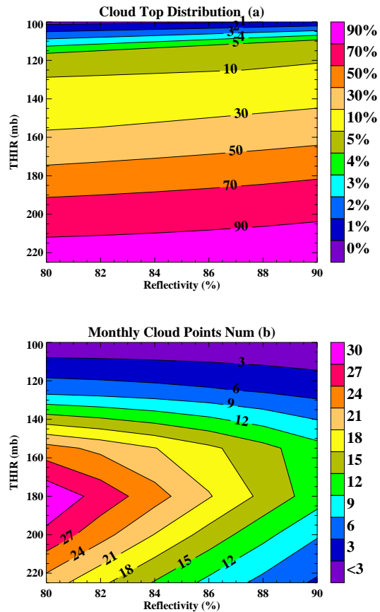
Fig. 3. (a) The THIR cloud-top distribution as a function of reflectivity for pressures less than 225 hPa, and (b) the monthly average number of cloud points between 1979–1984 as functions of THIR pressure and reflectivity.
