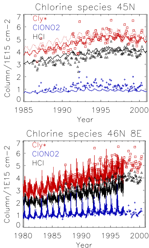
Fig. 1. Comparison of ground-based FTIR observations of HCl, \text{ClONO}_2 and their sum (labelled \text{Cl}_y^* ) at the Jungfraujoch ( 46^\circ \text{N} , 8^\circ \text{E} ) with 2D and 3D model results. (top) Monthly mean observations compared with 2D model run TD (output every 20 days). The red dotted line is the model total inorganic chlorine ( \text{Cl}_y ). (bottom) Monthly mean observations compared with 3D model run A (output every 2 days). (The Jungfraujoch observations were provided by R. Zander and E. Mahieu).
